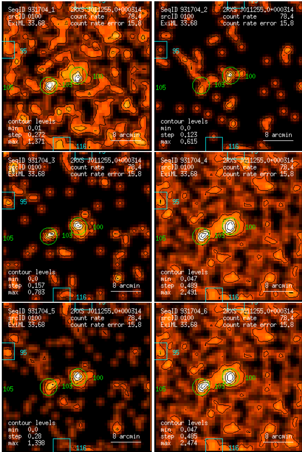
Figure 100: RASS 931704: detection 0100: band rate images, Gaussian filter: (1) PSPC channels 11 – 41, (2) 52 – 90, (3) 91 – 201, (4) 11 – 235, (5) 52 – 201, (6) 11 – 201. Broad band rates in counts/ks. Band rate contour levels in counts/ks/arcmin 2 .
