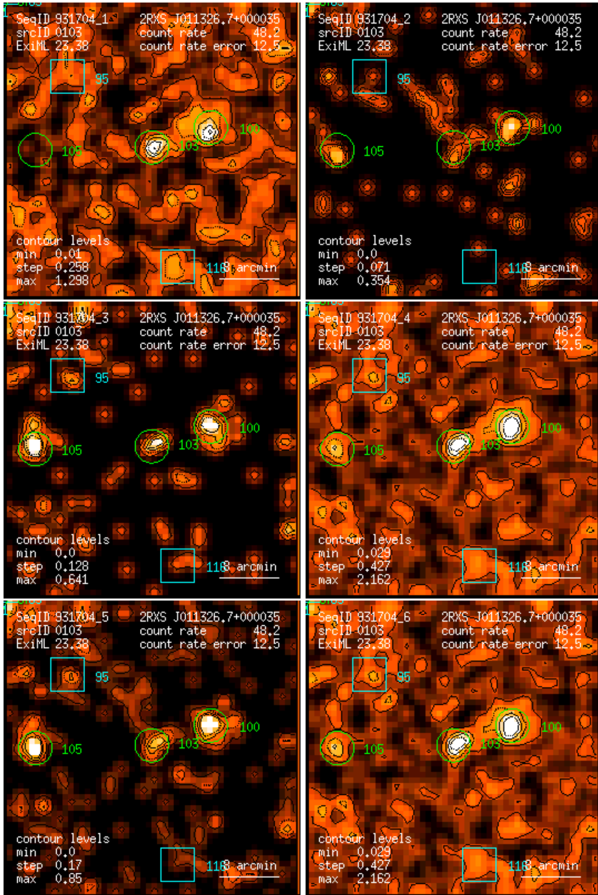
Figure 103: RASS 931704: detection 0103: band rate images, Gaussian filter: (1) PSPC channels 11 – 41, (2) 52 – 90, (3) 91 – 201, (4) 11 – 235, (5) 52 – 201, (6) 11 – 201. Broad band rates in counts/ks. Band rate contour levels in counts/ks/arcmin 2 .
