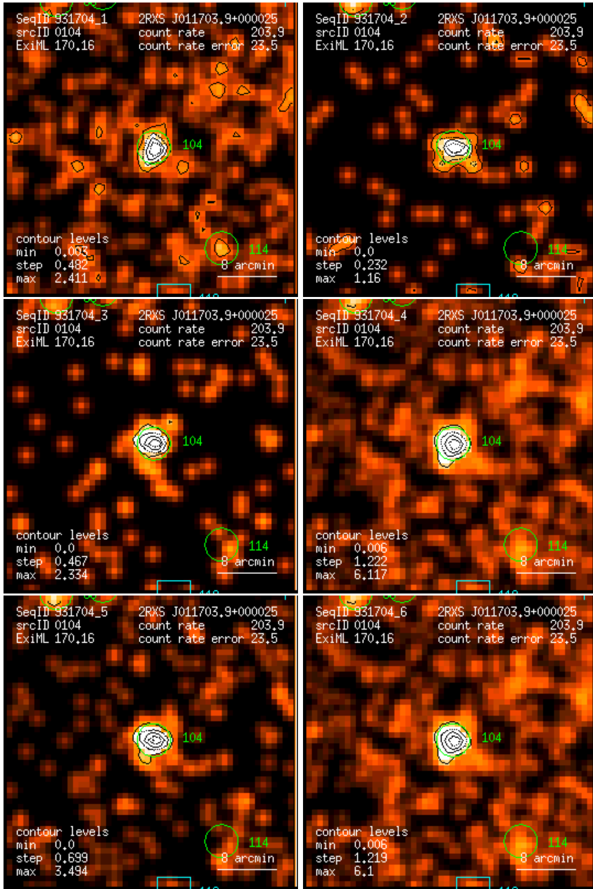
Figure 104: RASS 931704: detection 0104: band rate images, Gaussian filter: (1) PSPC channels 11 – 41, (2) 52 – 90, (3) 91 – 201, (4) 11 – 235, (5) 52 – 201, (6) 11 – 201. Broad band rates in counts/ks. Band rate contour levels in counts/ks/arcmin 2 .
