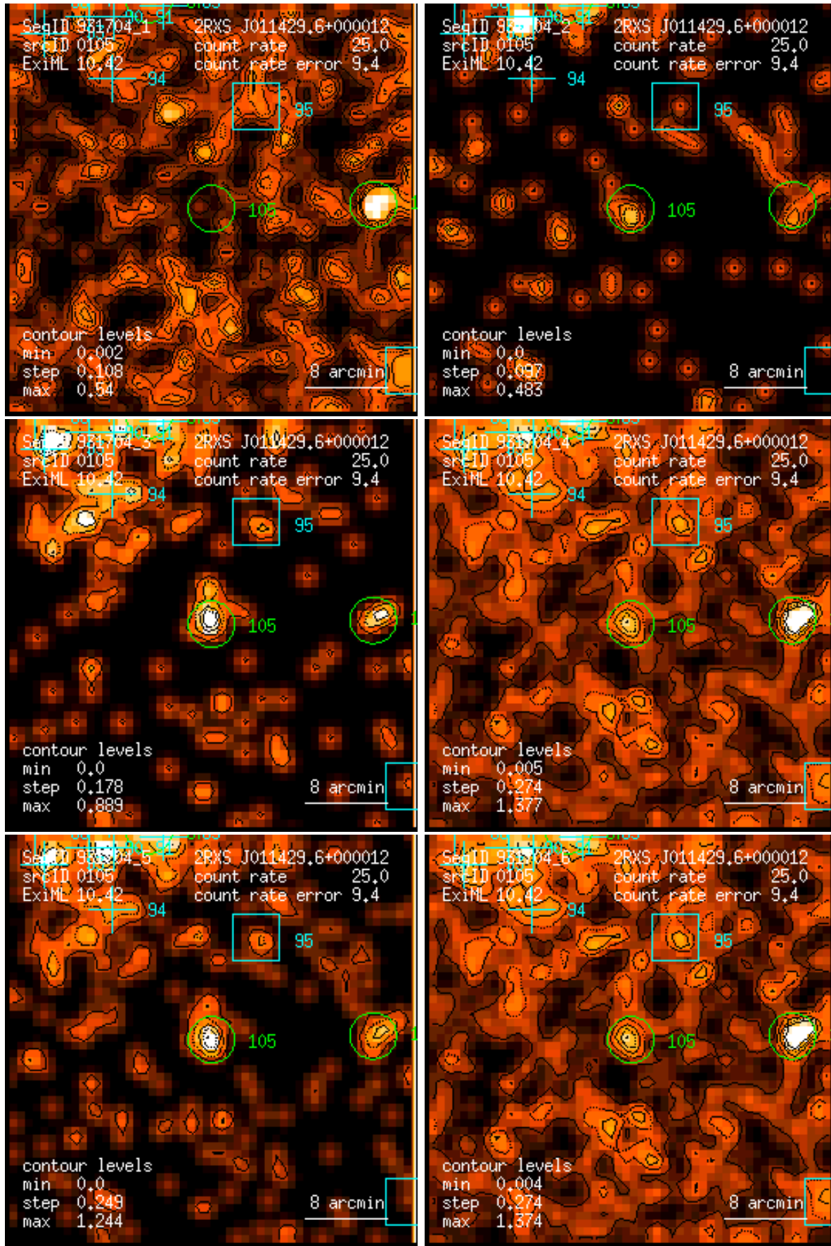
Figure 105: RASS 931704: detection 0105: band rate images, Gaussian filter: (1) PSPC channels 11 – 41, (2) 52 – 90, (3) 91 – 201, (4) 11 – 235, (5) 52 – 201, (6) 11 – 201. Broad band rates in counts/ks. Band rate contour levels in counts/ks/arcmin 2 .
