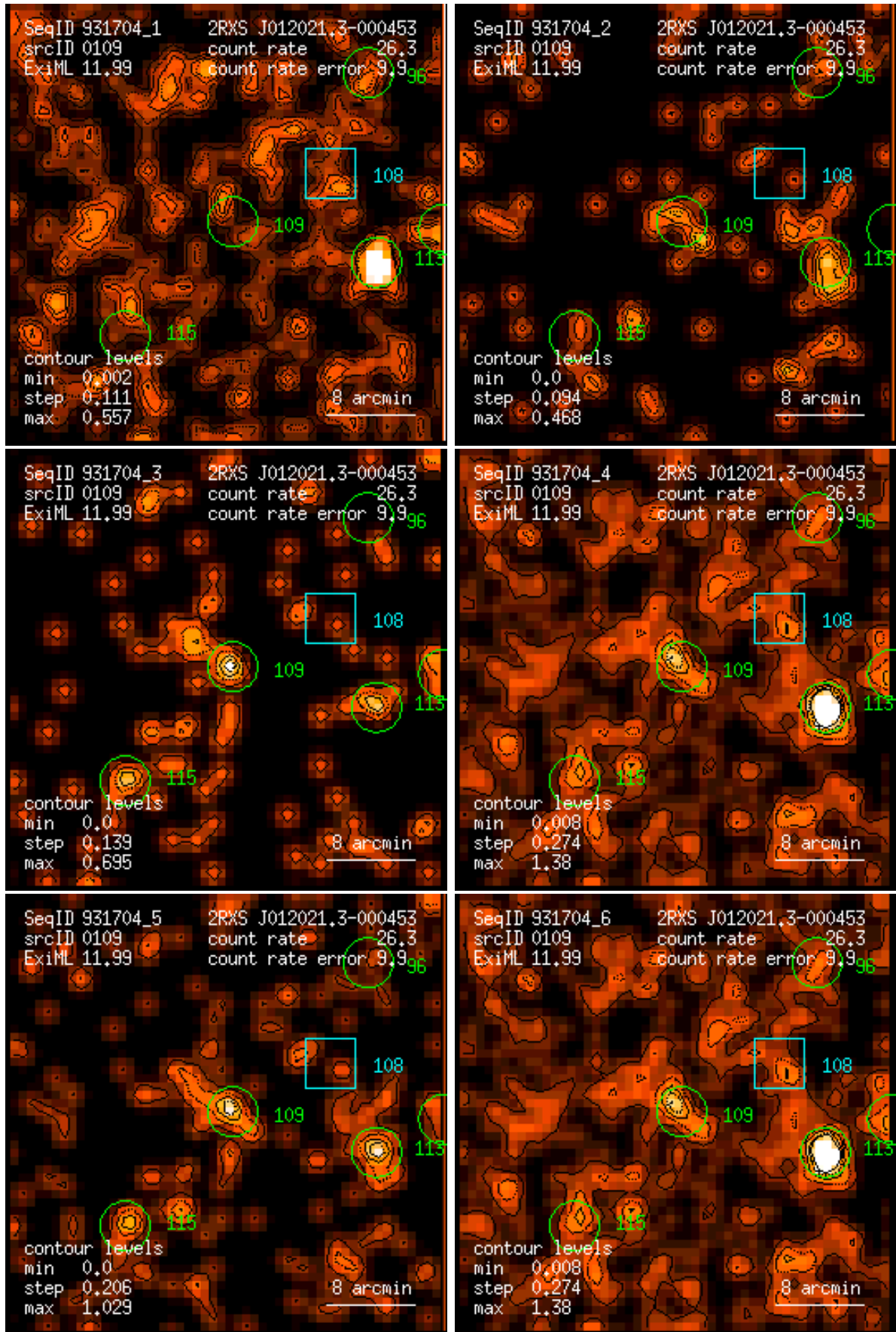
Figure 109: RASS 931704: detection 0109: band rate images, Gaussian filter: (1) PSPC channels 11 – 41, (2) 52 – 90, (3) 91 – 201, (4) 11 – 235, (5) 52 – 201, (6) 11 – 201. Broad band rates in counts/ks. Band rate contour levels in counts/ks/arcmin 2 .
