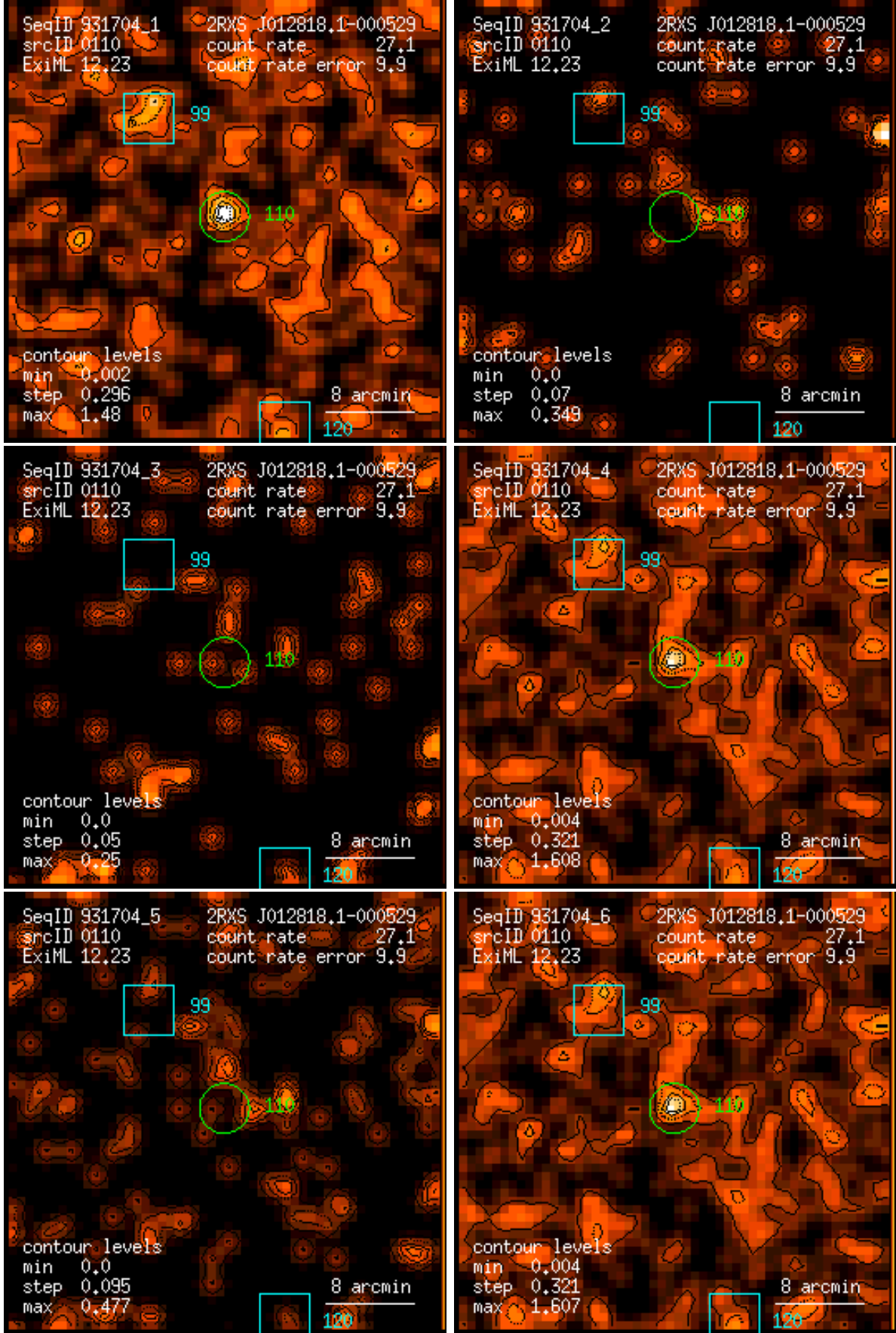
Figure 110: RASS 931704: detection 0110: band rate images, Gaussian filter: (1) PSPC channels 11 – 41, (2) 52 – 90, (3) 91 – 201, (4) 11 – 235, (5) 52 – 201, (6) 11 – 201. Broad band rates in counts/ks. Band rate contour levels in counts/ks/arcmin 2 .
