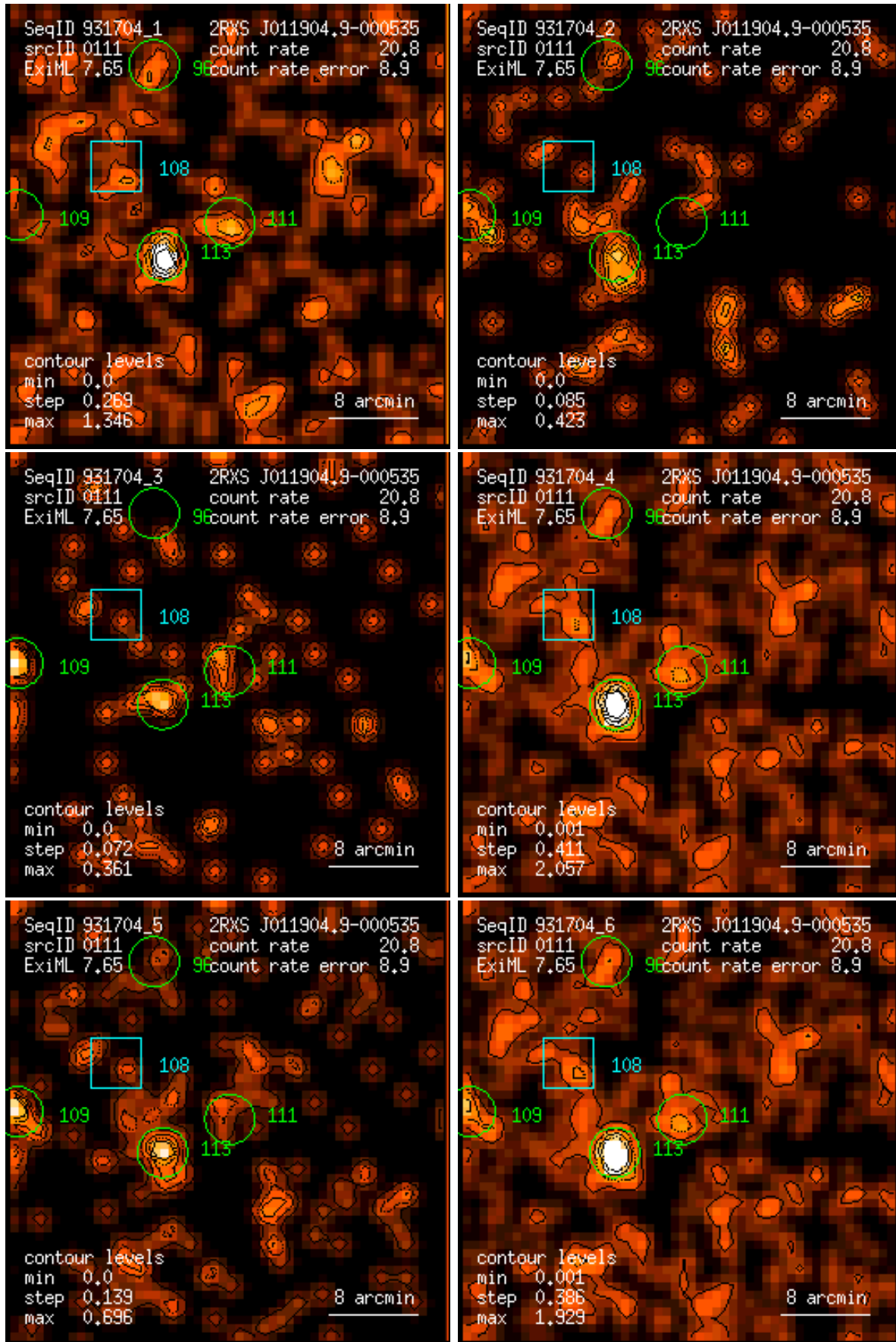
Figure 111: RASS 931704: detection 0111: band rate images, Gaussian filter: (1) PSPC channels 11 – 41, (2) 52 – 90, (3) 91 – 201, (4) 11 – 235, (5) 52 – 201, (6) 11 – 201. Broad band rates in counts/ks. Band rate contour levels in counts/ks/arcmin 2 .
