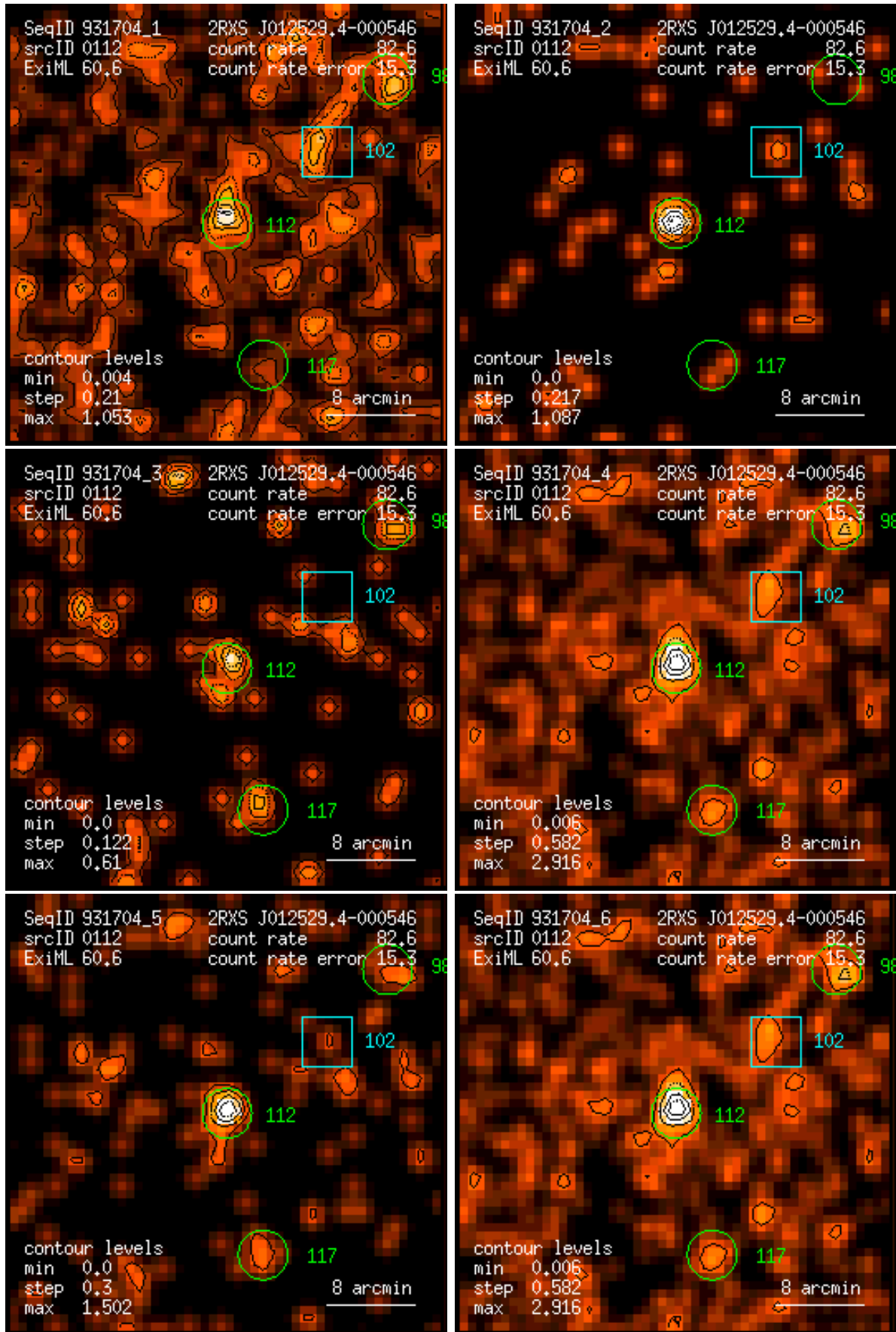
Figure 112: RASS 931704: detection 0112: band rate images, Gaussian filter: (1) PSPC channels 11 – 41, (2) 52 – 90, (3) 91 – 201, (4) 11 – 235, (5) 52 – 201, (6) 11 – 201. Broad band rates in counts/ks. Band rate contour levels in counts/ks/arcmin 2 .
