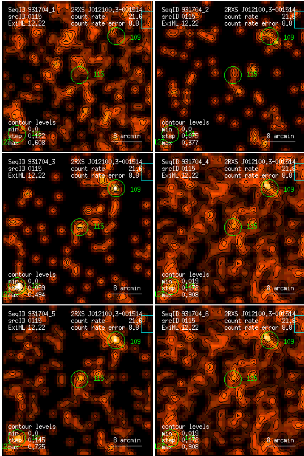
Figure 115: RASS 931704: detection 0115: band rate images, Gaussian filter: (1) PSPC channels 11 – 41, (2) 52 – 90, (3) 91 – 201, (4) 11 – 235, (5) 52 – 201, (6) 11 – 201. Broad band rates in counts/ks. Band rate contour levels in counts/ks/arcmin 2 .
