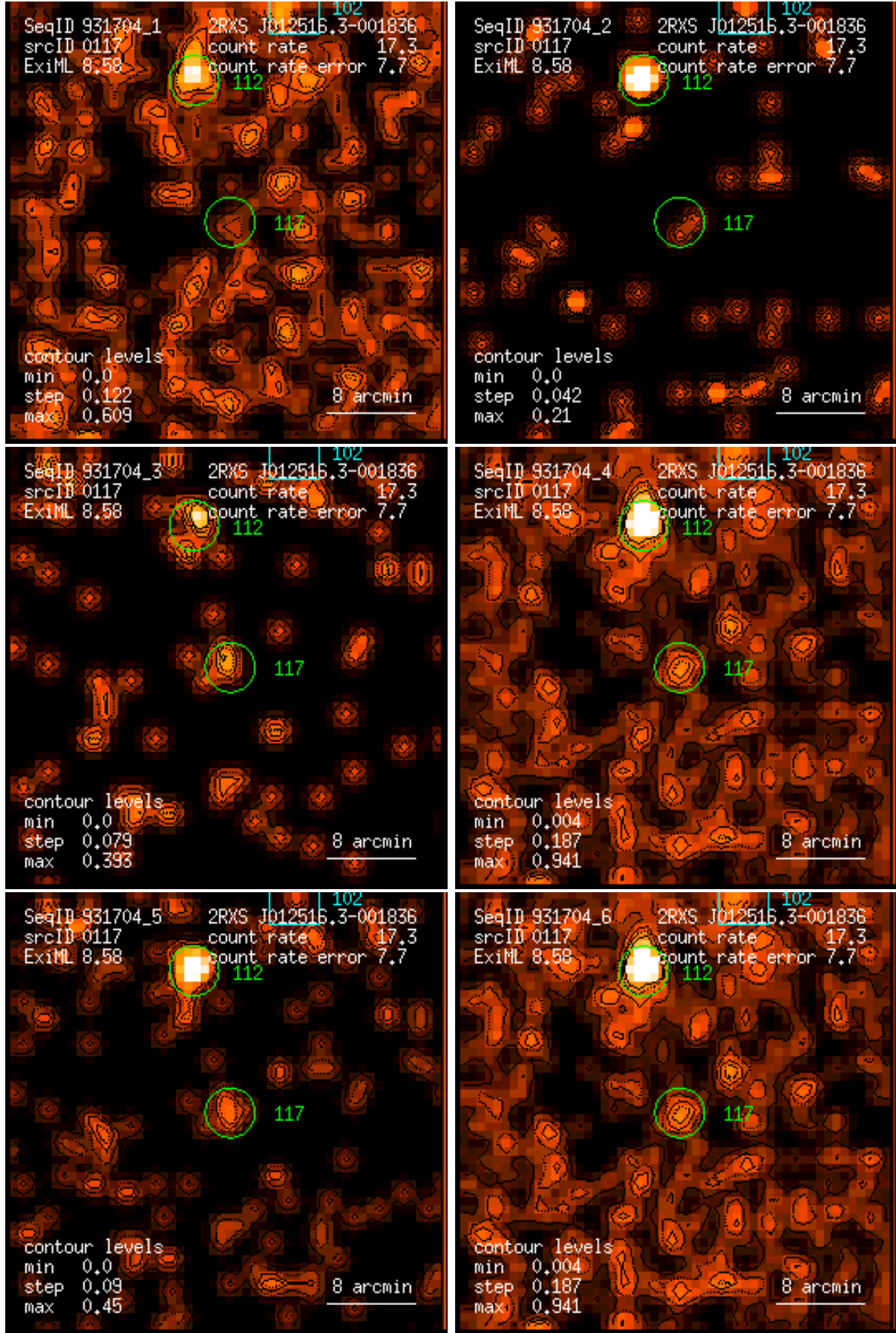
Figure 117: RASS 931704: detection 0117: band rate images, Gaussian filter: (1) PSPC channels 11 – 41, (2) 52 – 90, (3) 91 – 201, (4) 11 – 235, (5) 52 – 201, (6) 11 – 201. Broad band rates in counts/ks. Band rate contour levels in counts/ks/arcmin 2 .
