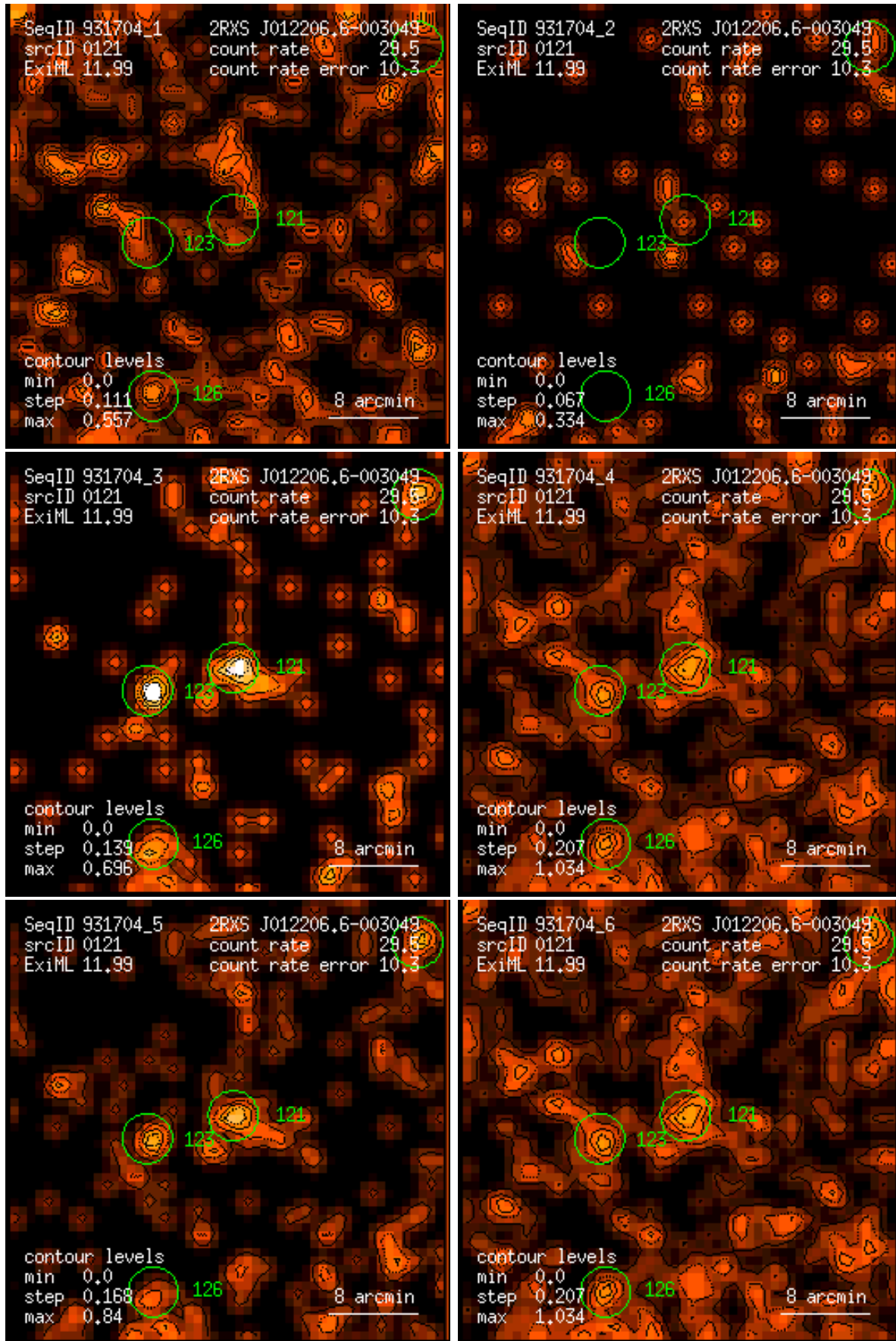
Figure 121: RASS 931704: detection 0121: band rate images, Gaussian filter: (1) PSPC channels 11 – 41, (2) 52 – 90, (3) 91 – 201, (4) 11 – 235, (5) 52 – 201, (6) 11 – 201. Broad band rates in counts/ks. Band rate contour levels in counts/ks/arcmin 2 .
