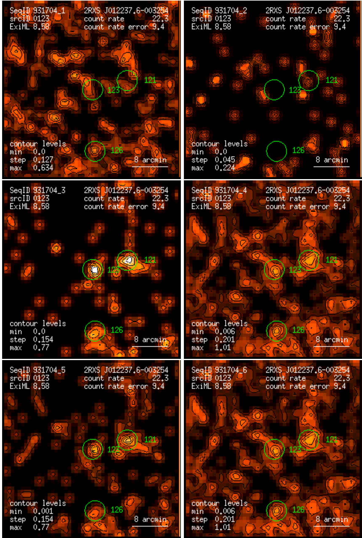
Figure 123: RASS 931704: detection 0123: band rate images, Gaussian filter: (1) PSPC channels 11 – 41, (2) 52 – 90, (3) 91 – 201, (4) 11 – 235, (5) 52 – 201, (6) 11 – 201. Broad band rates in counts/ks. Band rate contour levels in counts/ks/arcmin 2 .
