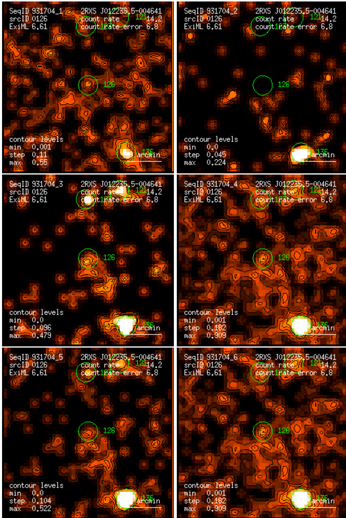
Figure 126: RASS 931704: detection 0126: band rate images, Gaussian filter: (1) PSPC channels 11 – 41, (2) 52 – 90, (3) 91 – 201, (4) 11 – 235, (5) 52 – 201, (6) 11 – 201. Broad band rates in counts/ks. Band rate contour levels in counts/ks/arcmin 2 .
