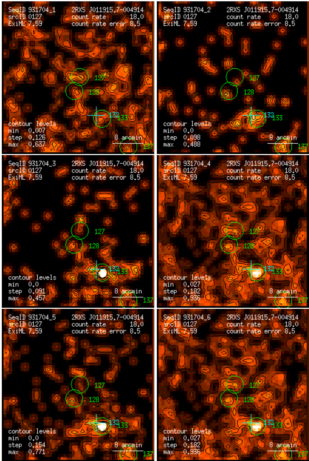
Figure 127: RASS 931704: detection 0127: band rate images, Gaussian filter: (1) PSPC channels 11 – 41, (2) 52 – 90, (3) 91 – 201, (4) 11 – 235, (5) 52 – 201, (6) 11 – 201. Broad band rates in counts/ks. Band rate contour levels in counts/ks/arcmin 2 .
