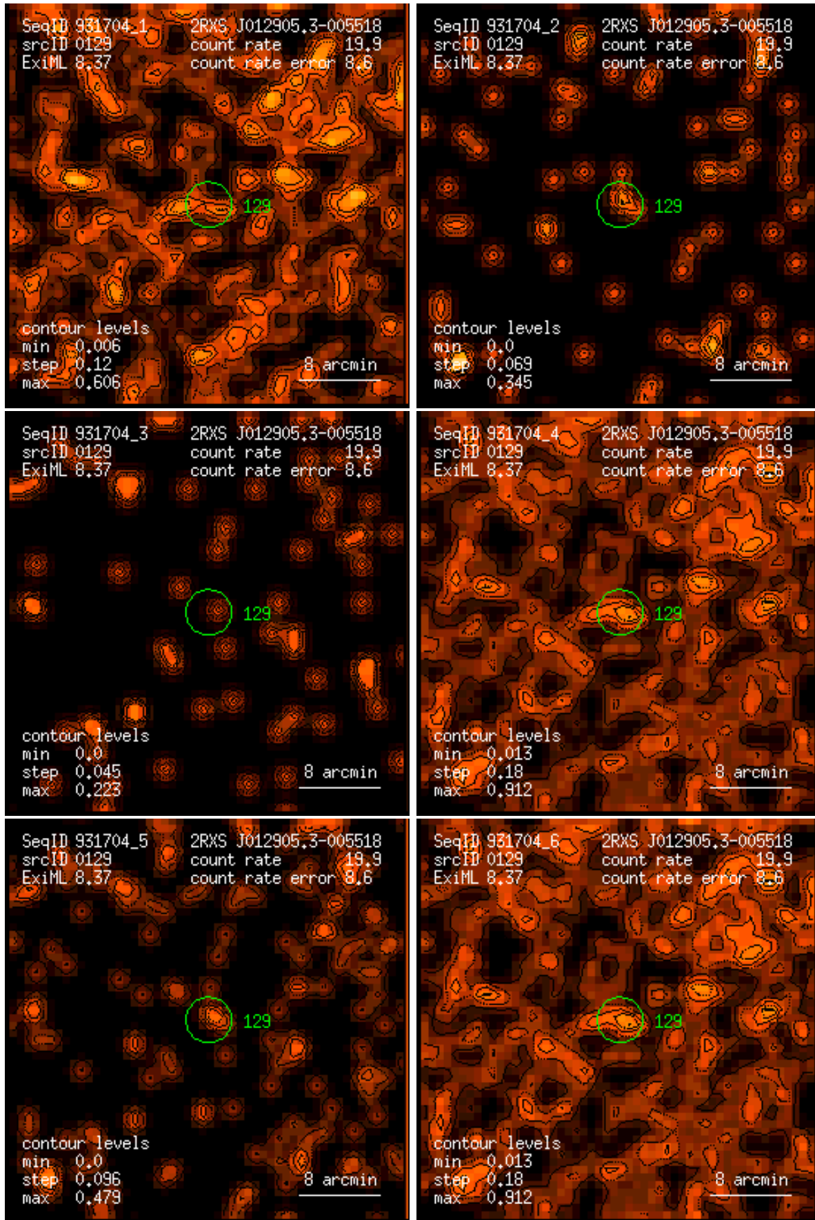
Figure 129: RASS 931704: detection 0129: band rate images, Gaussian filter: (1) PSPC channels 11 – 41, (2) 52 – 90, (3) 91 – 201, (4) 11 – 235, (5) 52 – 201, (6) 11 – 201. Broad band rates in counts/ks. Band rate contour levels in counts/ks/arcmin 2 .
