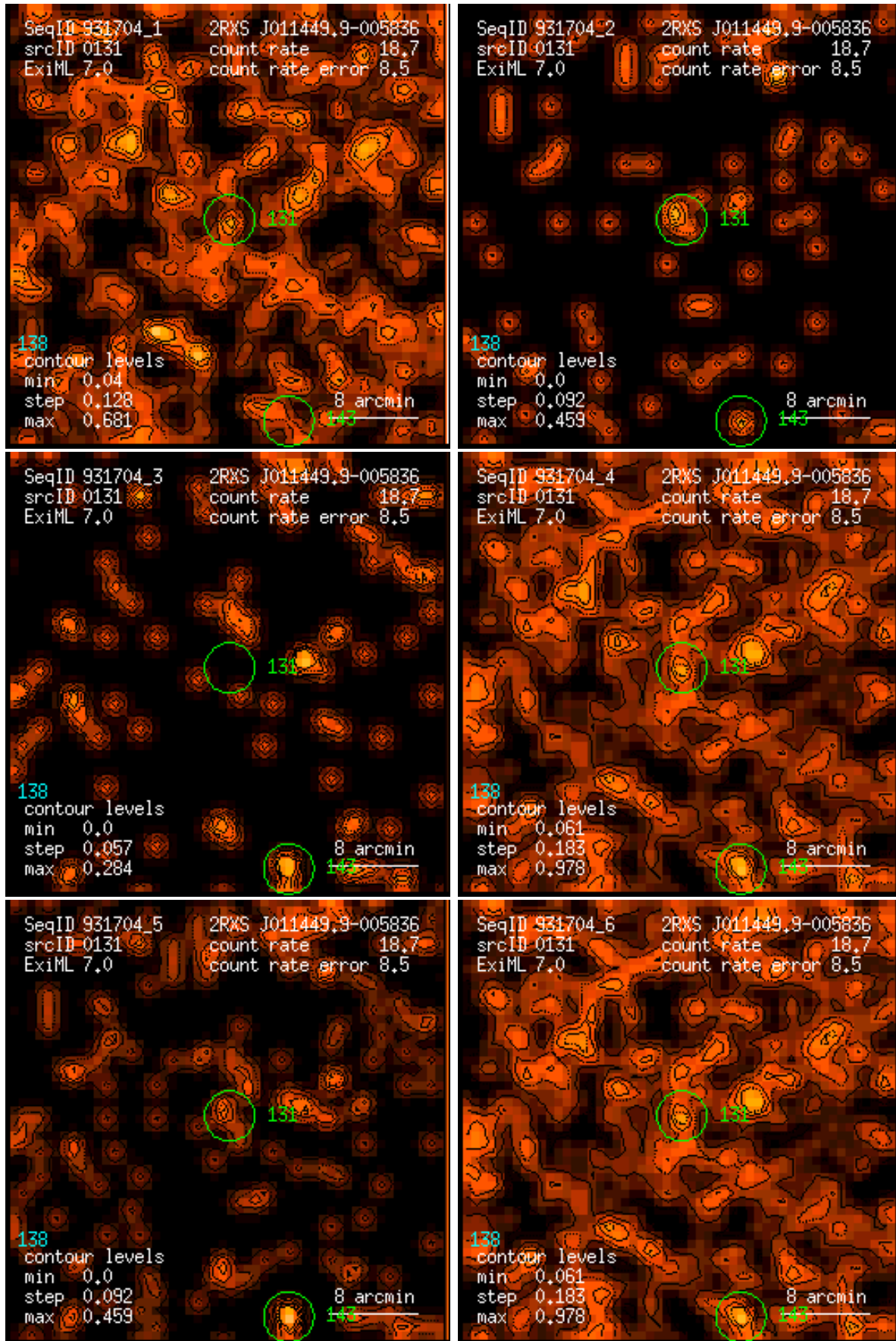
Figure 131: RASS 931704: detection 0131: band rate images, Gaussian filter: (1) PSPC channels 11 – 41, (2) 52 – 90, (3) 91 – 201, (4) 11 – 235, (5) 52 – 201, (6) 11 – 201. Broad band rates in counts/ks. Band rate contour levels in counts/ks/arcmin 2 .
