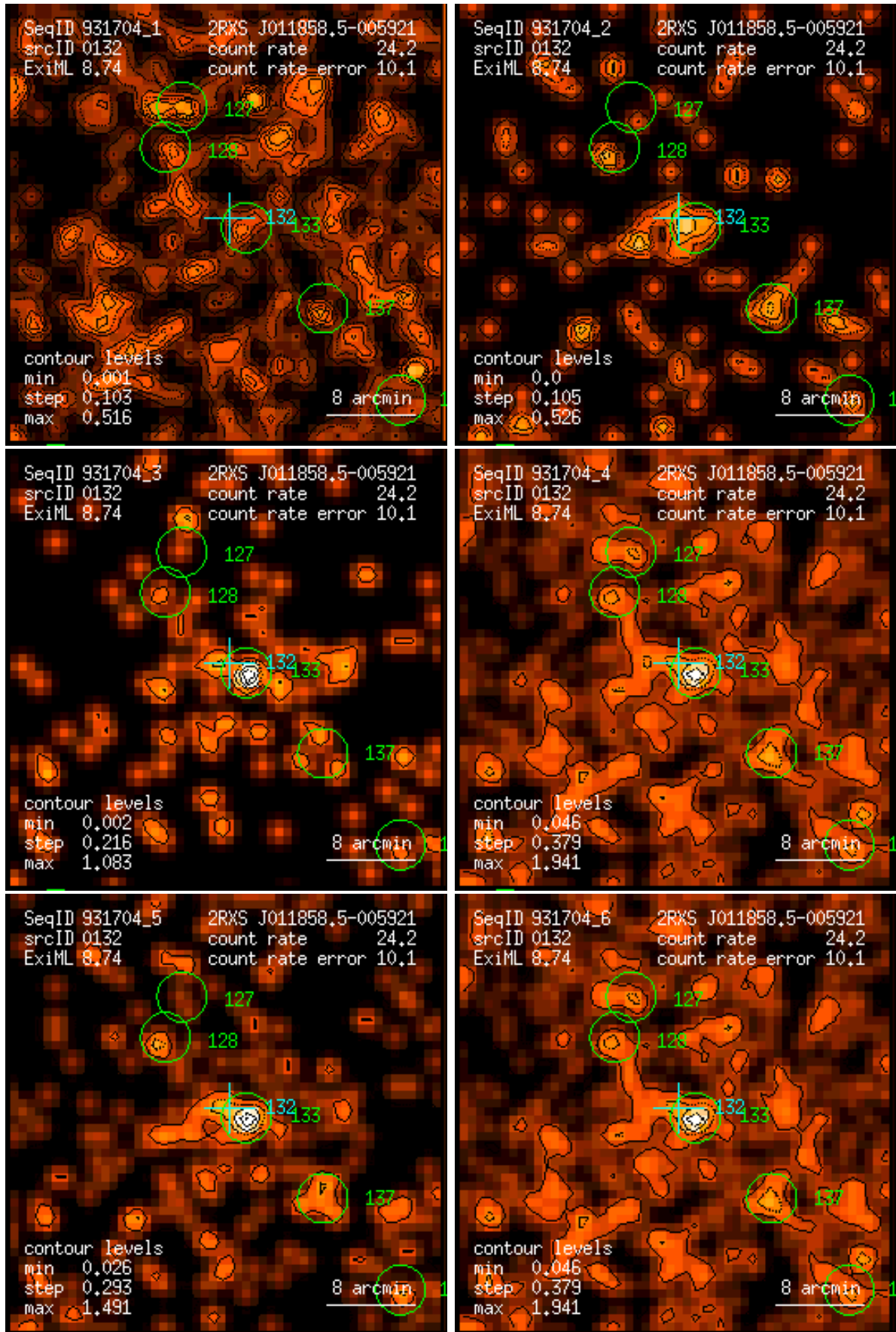
Figure 132: RASS 931704: detection 0132: band rate images, Gaussian filter: (1) PSPC channels 11 – 41, (2) 52 – 90, (3) 91 – 201, (4) 11 – 235, (5) 52 – 201, (6) 11 – 201. Broad band rates in counts/ks. Band rate contour levels in counts/ks/arcmin 2 .
