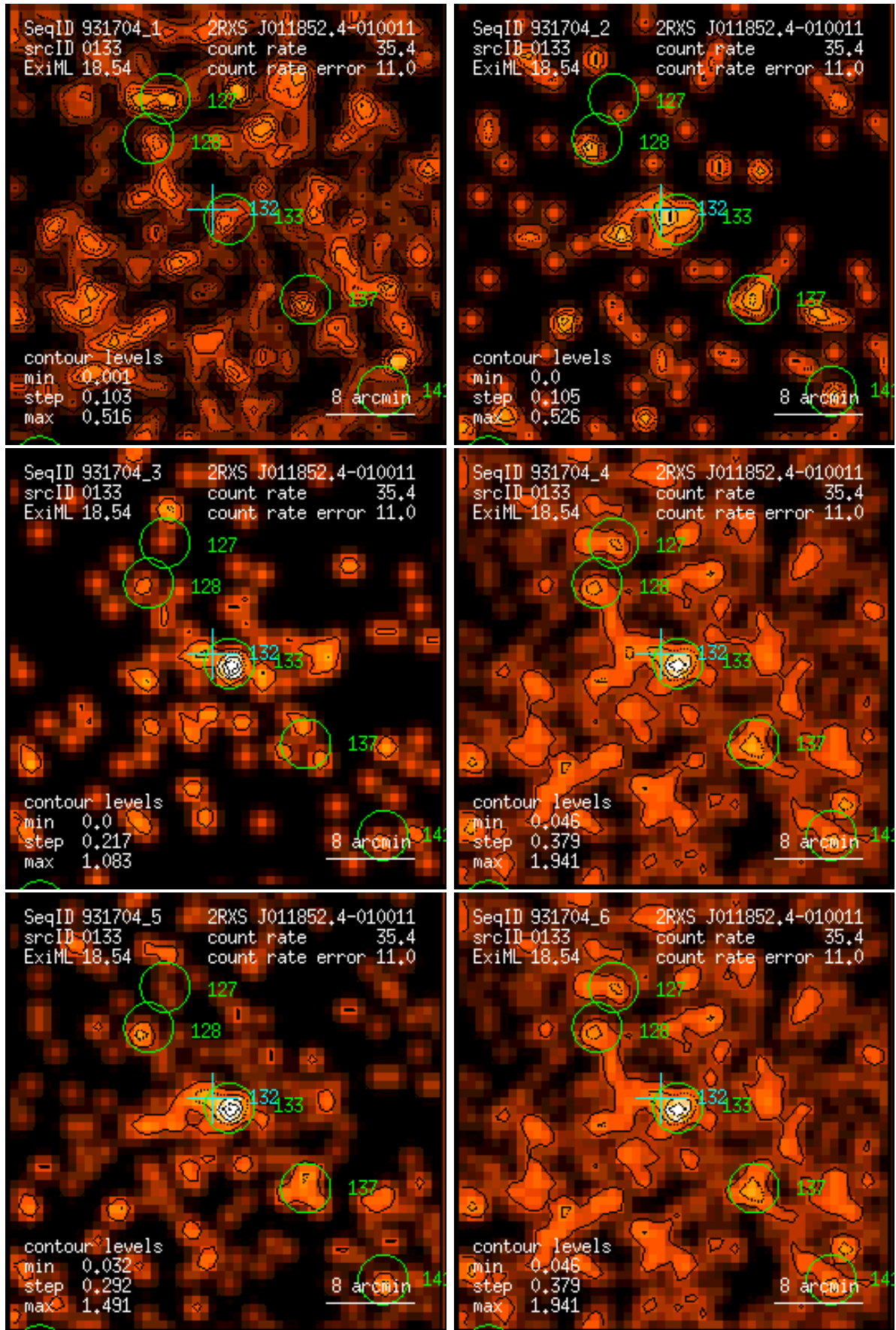
Figure 133: RASS 931704: detection 0133: band rate images, Gaussian filter: (1) PSPC channels 11 – 41, (2) 52 – 90, (3) 91 – 201, (4) 11 – 235, (5) 52 – 201, (6) 11 – 201. Broad band rates in counts/ks. Band rate contour levels in counts/ks/arcmin 2 .
