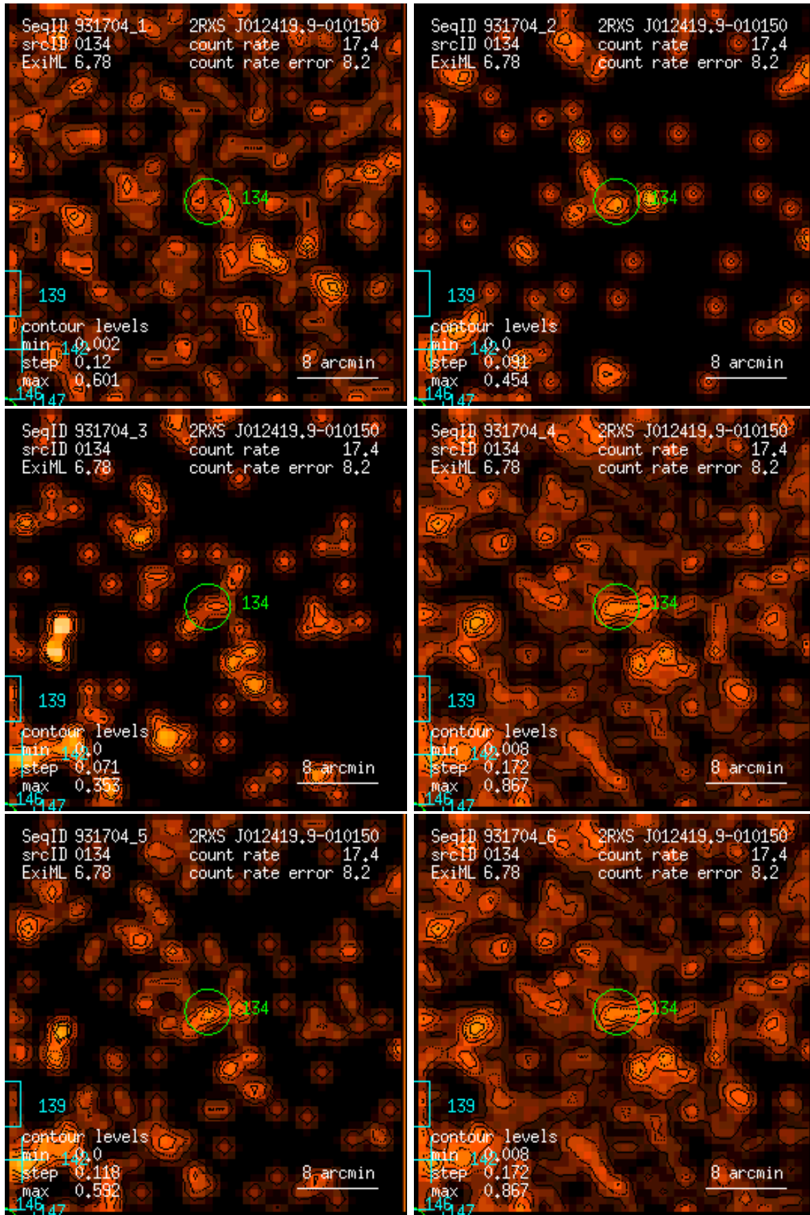
Figure 134: RASS 931704: detection 0134: band rate images, Gaussian filter: (1) PSPC channels 11 – 41, (2) 52 – 90, (3) 91 – 201, (4) 11 – 235, (5) 52 – 201, (6) 11 – 201. Broad band rates in counts/ks. Band rate contour levels in counts/ks/arcmin 2 .
