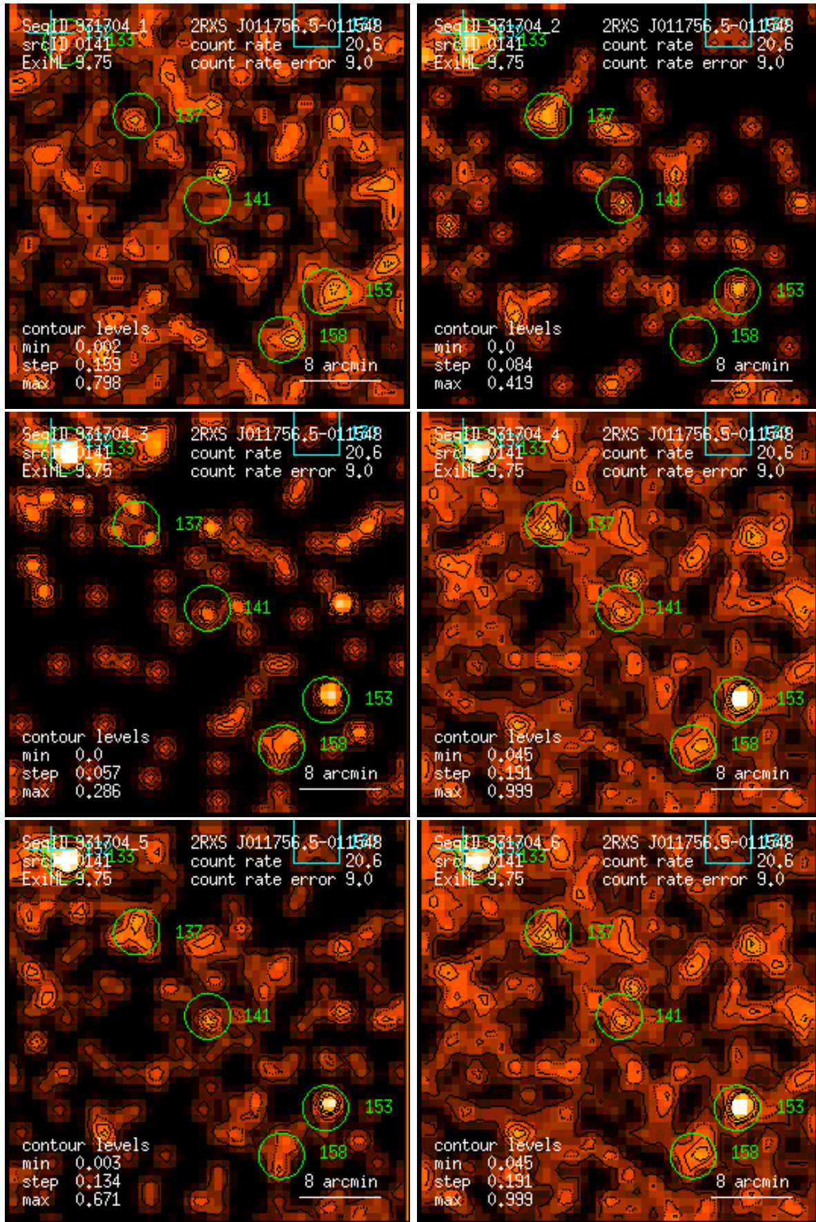
Figure 141: RASS 931704: detection 0141: band rate images, Gaussian filter: (1) PSPC channels 11 – 41, (2) 52 – 90, (3) 91 – 201, (4) 11 – 235, (5) 52 – 201, (6) 11 – 201. Broad band rates in counts/ks. Band rate contour levels in counts/ks/arcmin 2 .
