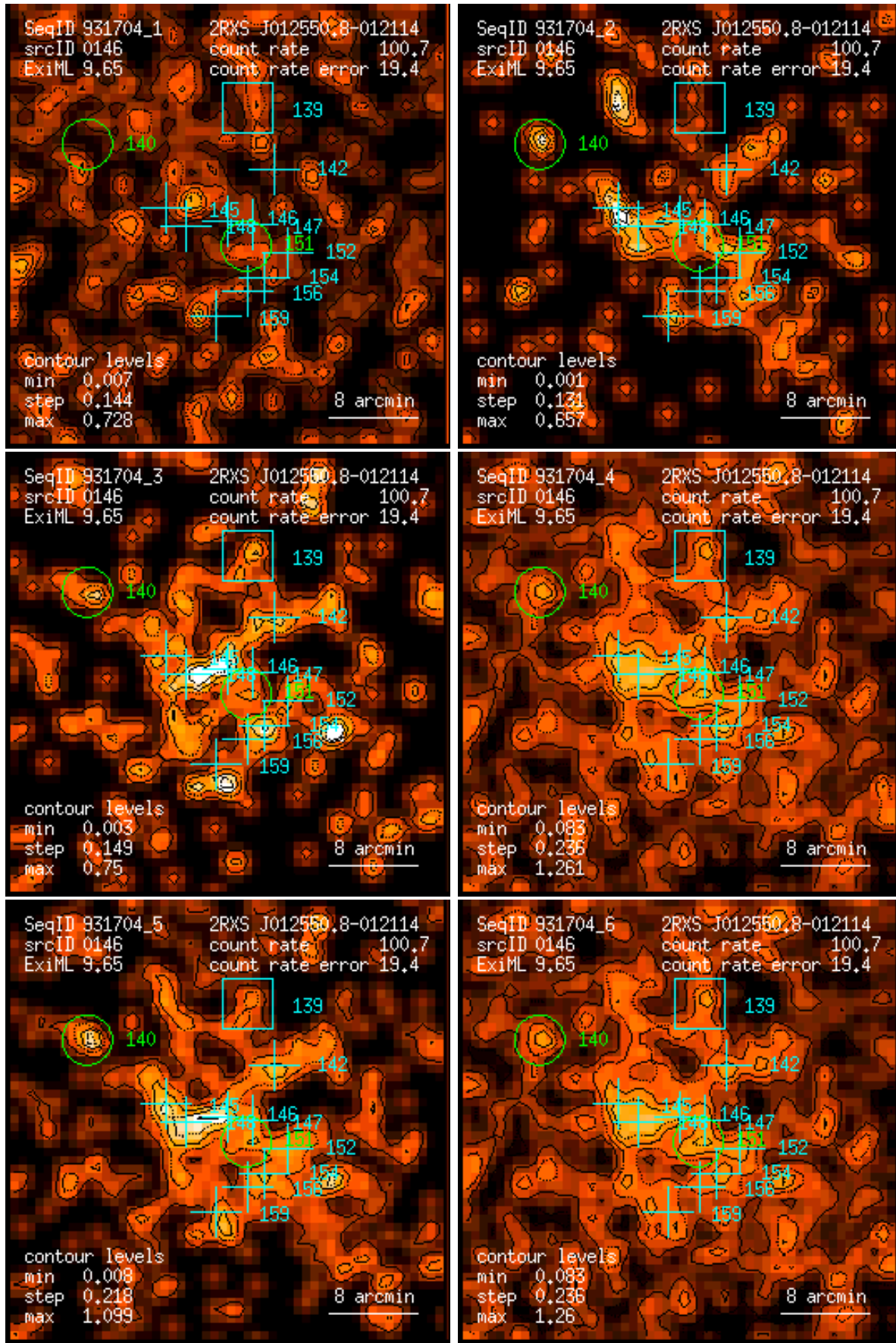
Figure 146: RASS 931704: detection 0146: band rate images, Gaussian filter: (1) PSPC channels 11 – 41, (2) 52 – 90, (3) 91 – 201, (4) 11 – 235, (5) 52 – 201, (6) 11 – 201. Broad band rates in counts/ks. Band rate contour levels in counts/ks/arcmin 2 .
