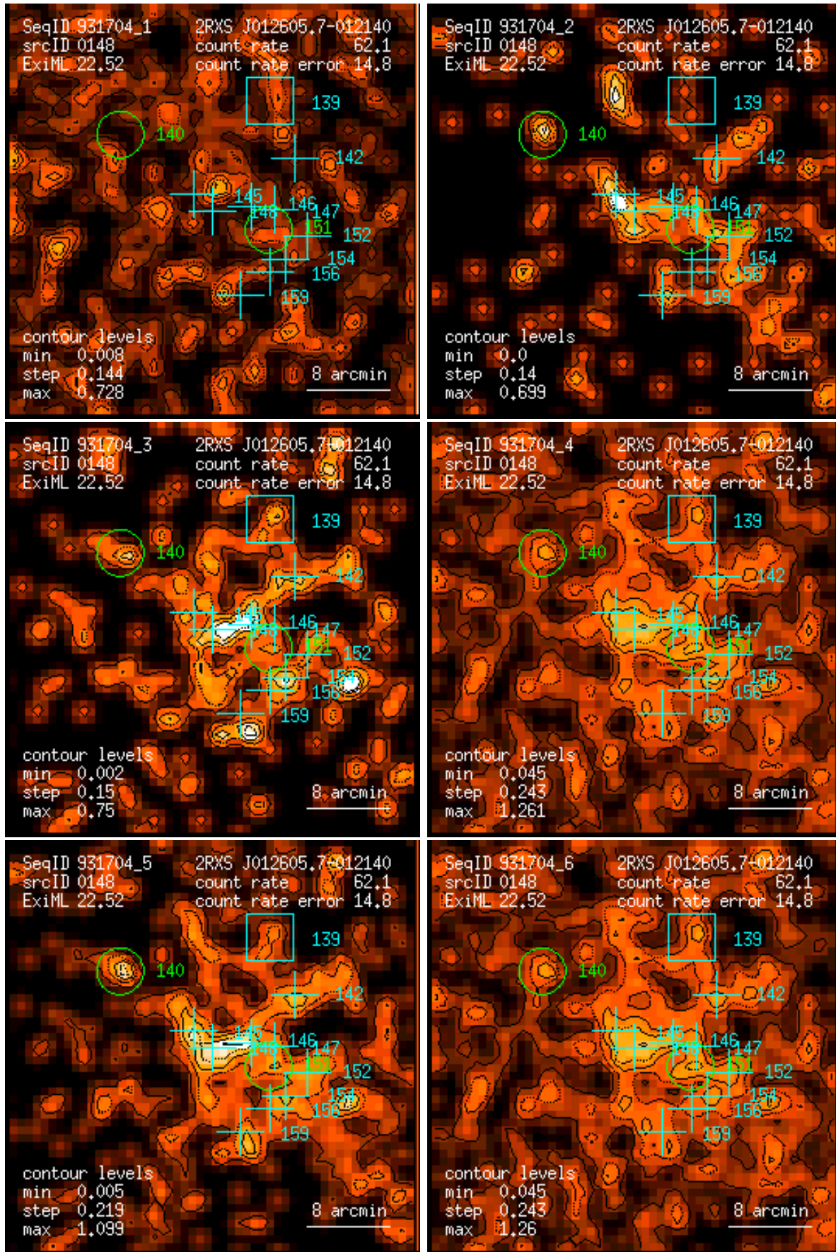
Figure 148: RASS 931704: detection 0148: band rate images, Gaussian filter: (1) PSPC channels 11 – 41, (2) 52 – 90, (3) 91 – 201, (4) 11 – 235, (5) 52 – 201, (6) 11 – 201. Broad band rates in counts/ks. Band rate contour levels in counts/ks/arcmin 2 .
