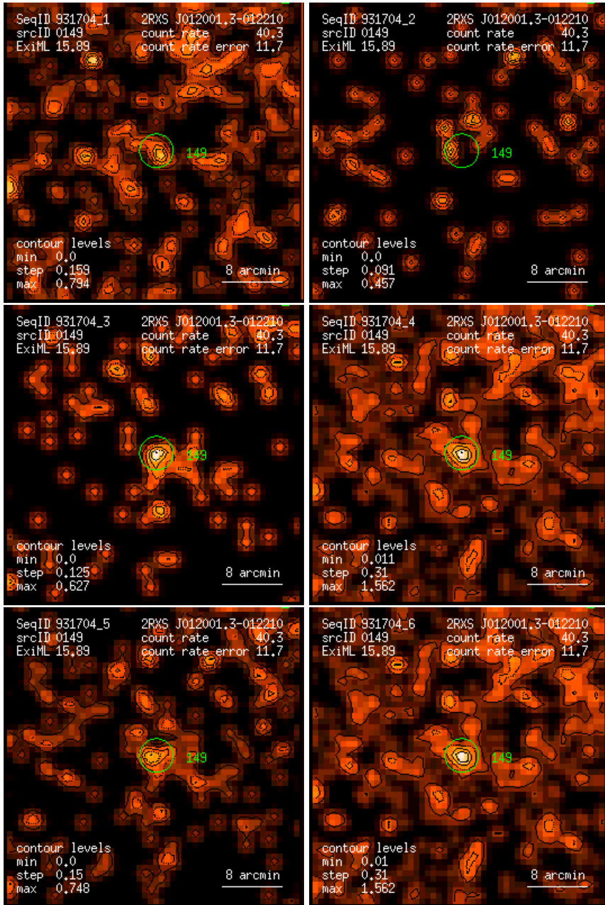
Figure 149: RASS 931704: detection 0149: band rate images, Gaussian filter: (1) PSPC channels 11 – 41, (2) 52 – 90, (3) 91 – 201, (4) 11 – 235, (5) 52 – 201, (6) 11 – 201. Broad band rates in counts/ks. Band rate contour levels in counts/ks/arcmin 2 .
