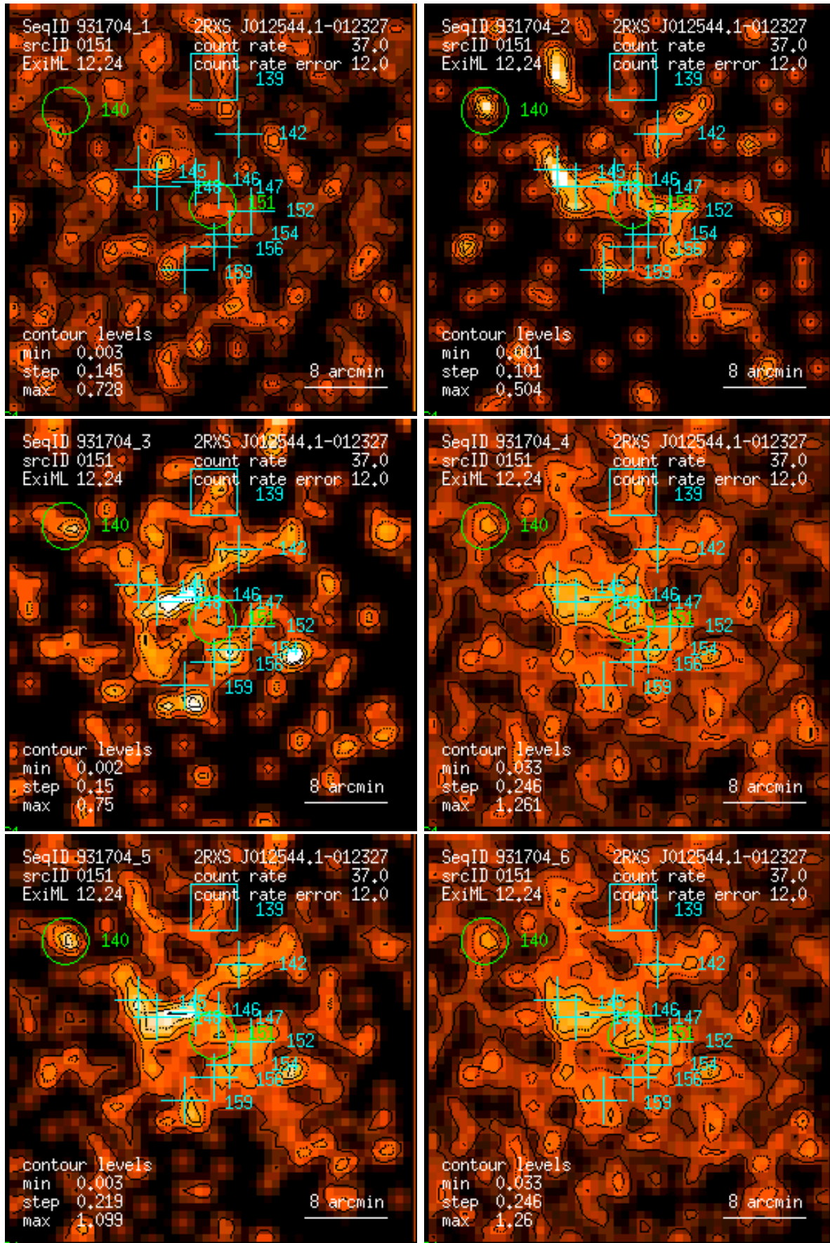
Figure 151: RASS 931704: detection 0151: band rate images, Gaussian filter: (1) PSPC channels 11 – 41, (2) 52 – 90, (3) 91 – 201, (4) 11 – 235, (5) 52 – 201, (6) 11 – 201. Broad band rates in counts/ks. Band rate contour levels in counts/ks/arcmin 2 .
