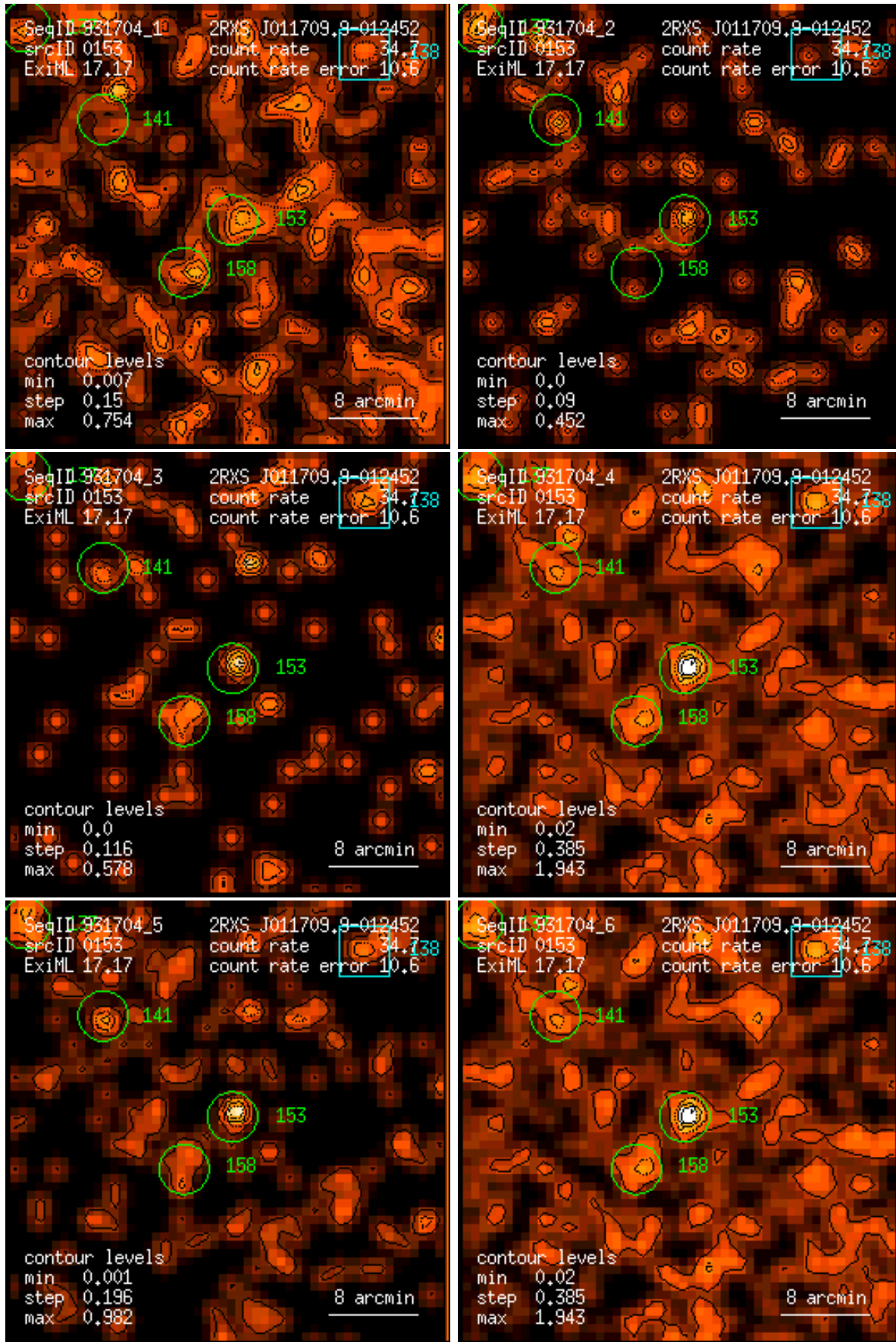
Figure 153: RASS 931704: detection 0153: band rate images, Gaussian filter: (1) PSPC channels 11 – 41, (2) 52 – 90, (3) 91 – 201, (4) 11 – 235, (5) 52 – 201, (6) 11 – 201. Broad band rates in counts/ks. Band rate contour levels in counts/ks/arcmin 2 .
