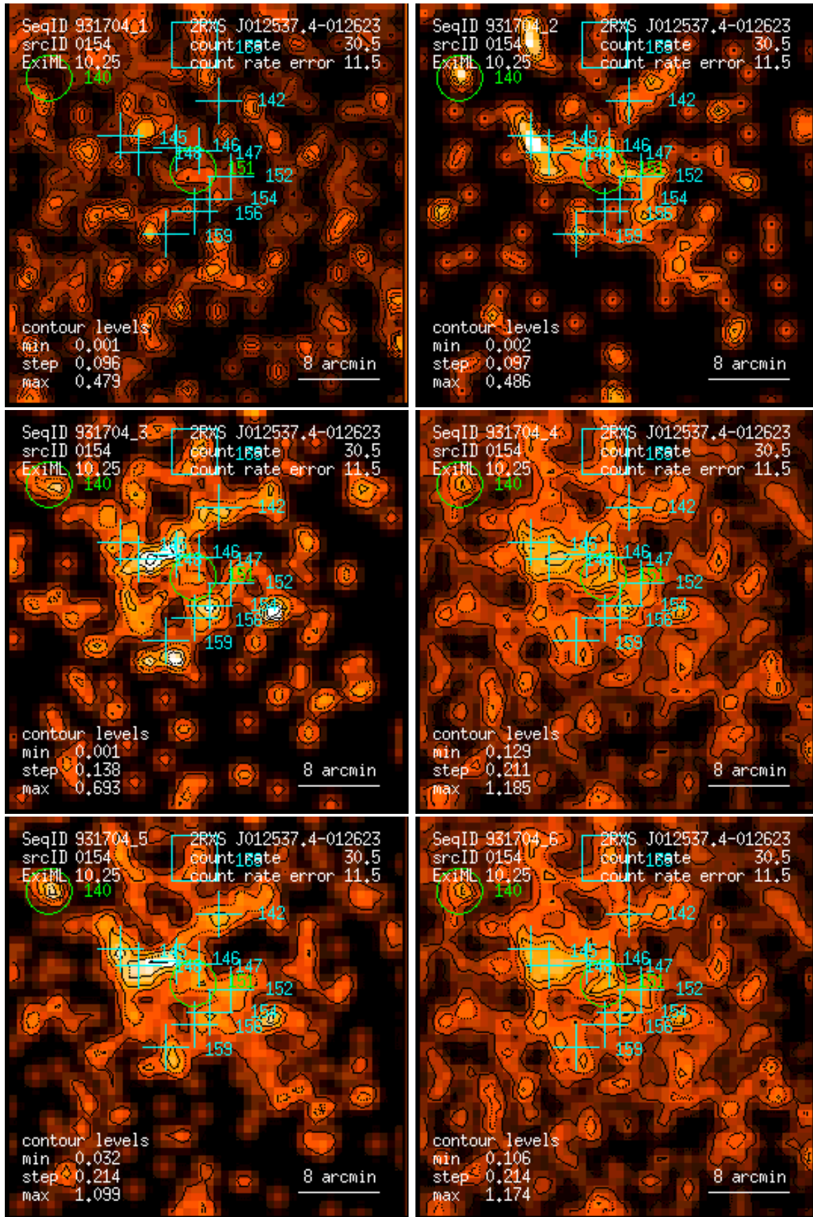
Figure 154: RASS 931704: detection 0154: band rate images, Gaussian filter: (1) PSPC channels 11 – 41, (2) 52 – 90, (3) 91 – 201, (4) 11 – 235, (5) 52 – 201, (6) 11 – 201. Broad band rates in counts/ks. Band rate contour levels in counts/ks/arcmin 2 .
