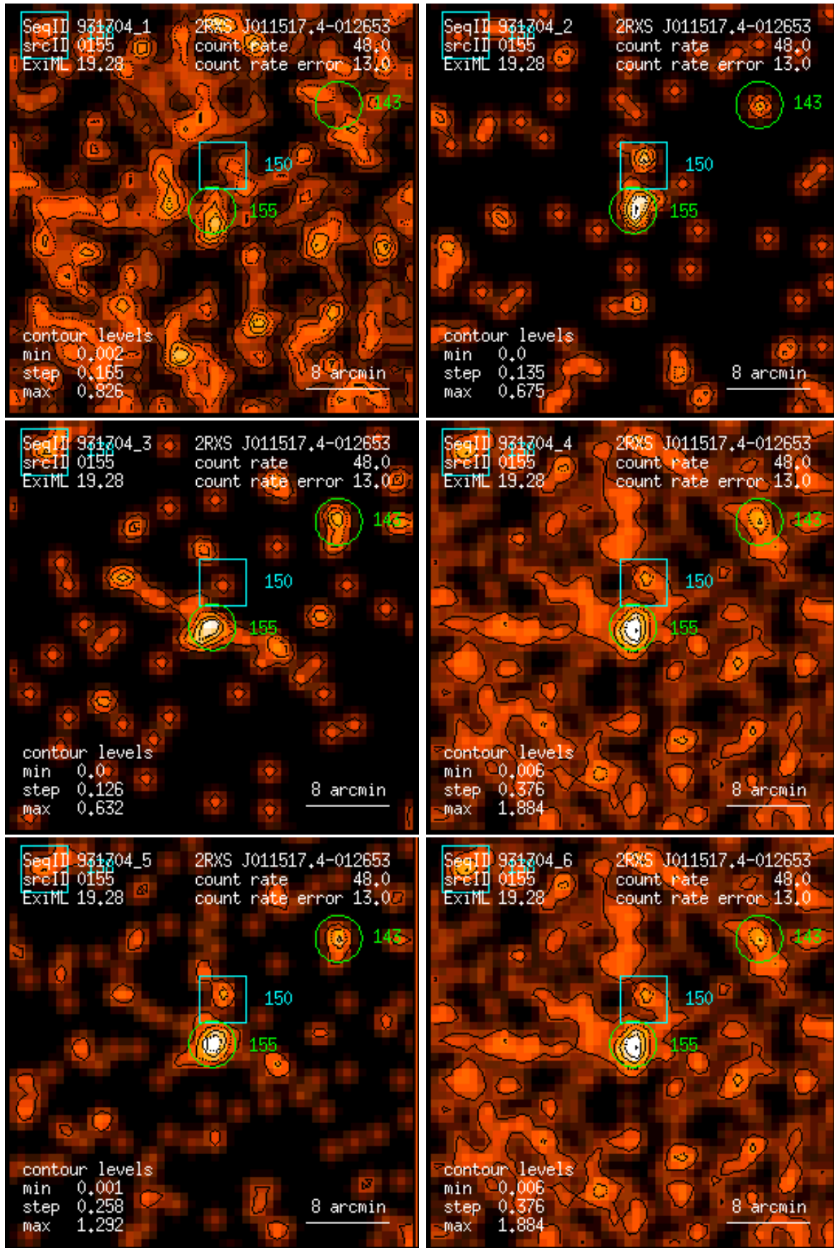
Figure 155: RASS 931704: detection 0155: band rate images, Gaussian filter: (1) PSPC channels 11 – 41, (2) 52 – 90, (3) 91 – 201, (4) 11 – 235, (5) 52 – 201, (6) 11 – 201. Broad band rates in counts/ks. Band rate contour levels in counts/ks/arcmin 2 .
