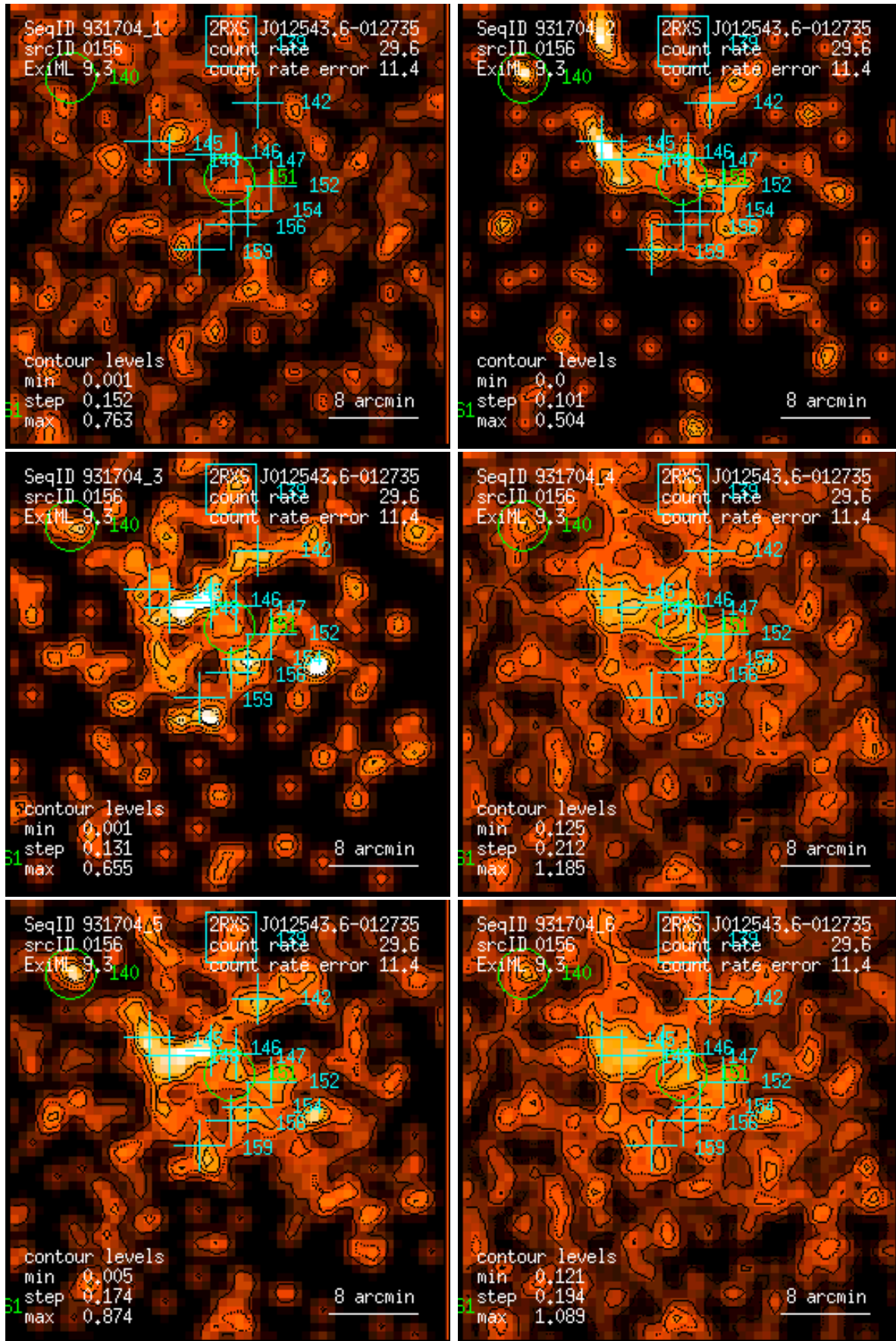
Figure 156: RASS 931704: detection 0156: band rate images, Gaussian filter: (1) PSPC channels 11 – 41, (2) 52 – 90, (3) 91 – 201, (4) 11 – 235, (5) 52 – 201, (6) 11 – 201. Broad band rates in counts/ks. Band rate contour levels in counts/ks/arcmin 2 .
