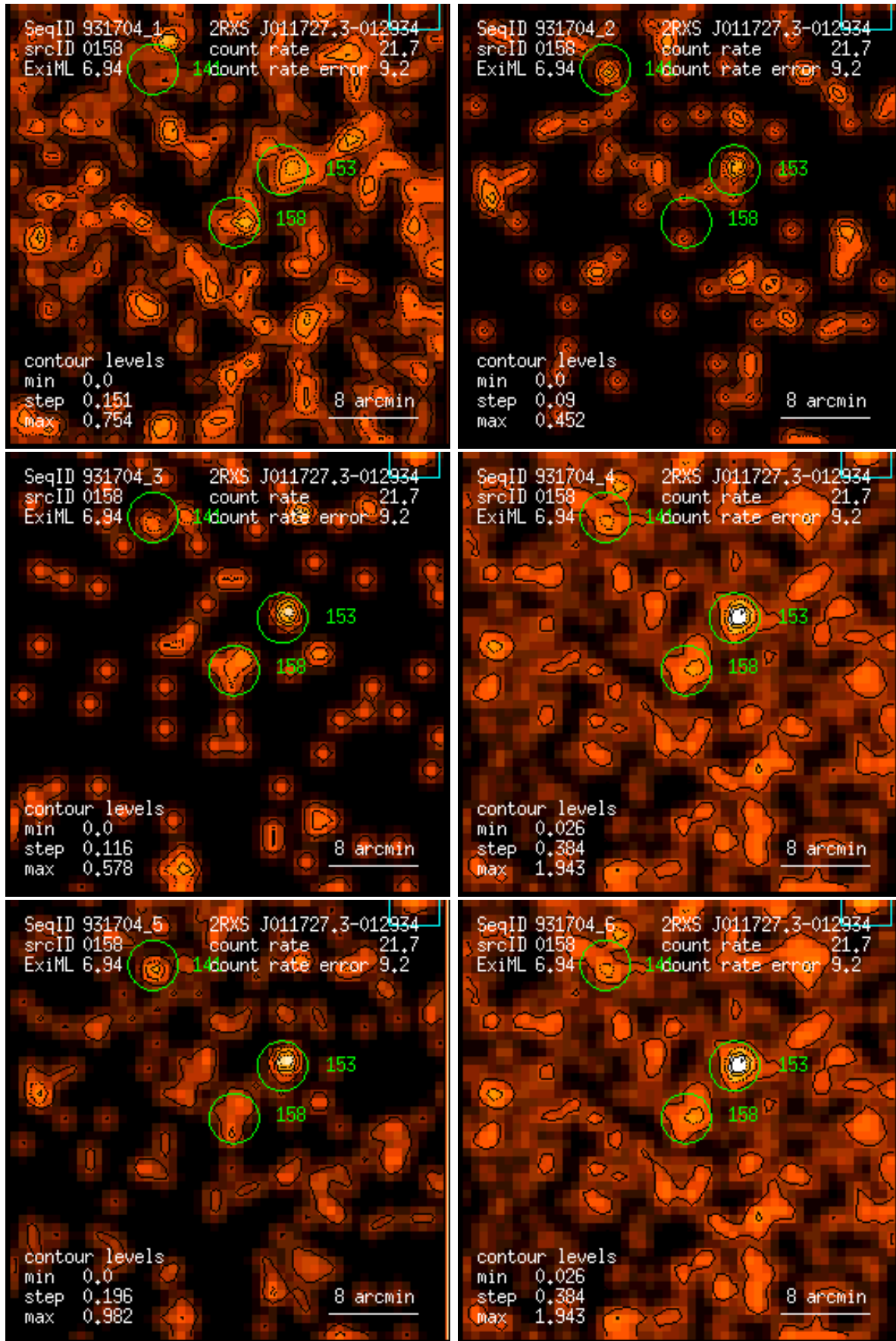
Figure 158: RASS 931704: detection 0158: band rate images, Gaussian filter: (1) PSPC channels 11 – 41, (2) 52 – 90, (3) 91 – 201, (4) 11 – 235, (5) 52 – 201, (6) 11 – 201. Broad band rates in counts/ks. Band rate contour levels in counts/ks/arcmin 2 .
