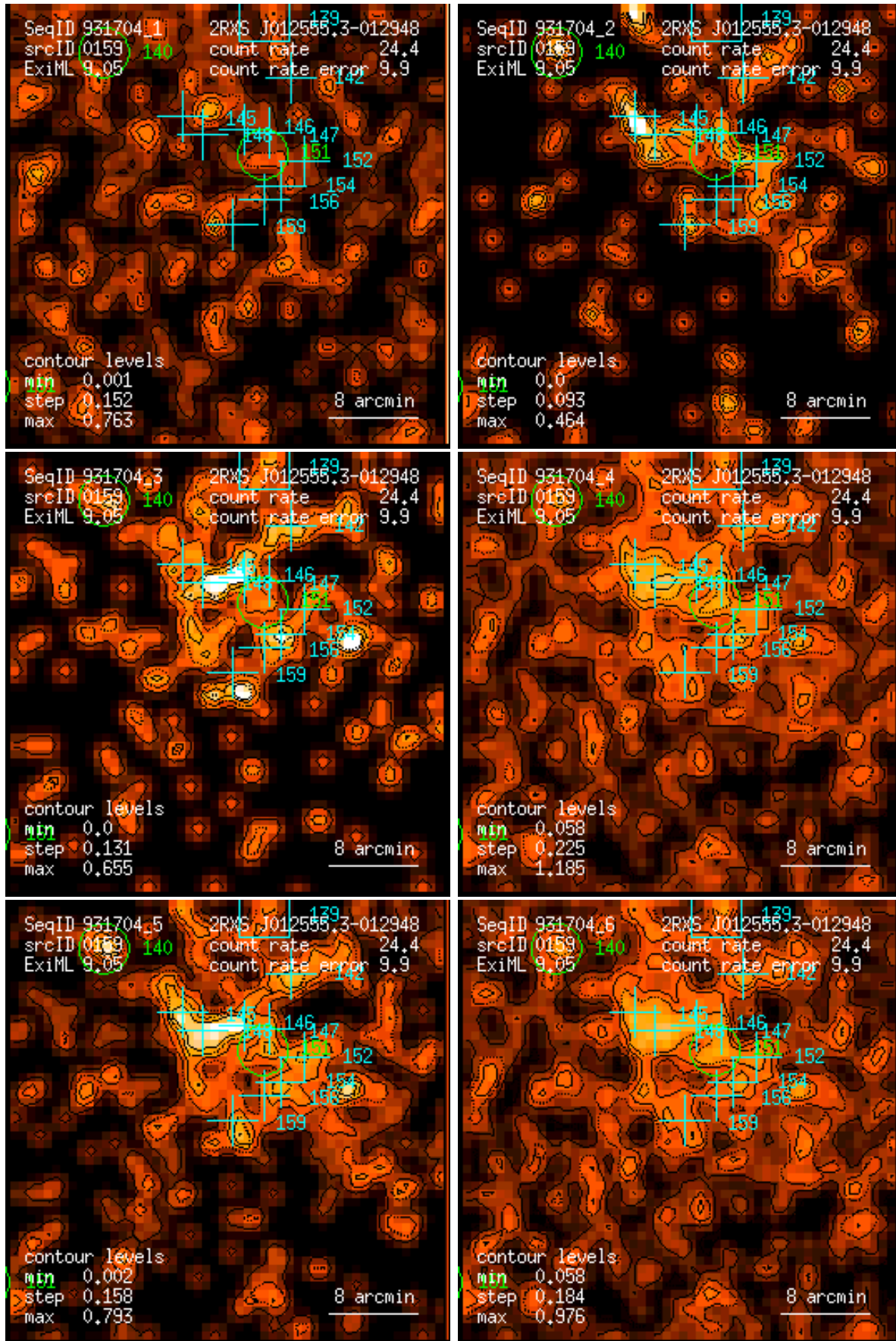
Figure 159: RASS 931704: detection 0159: band rate images, Gaussian filter: (1) PSPC channels 11 – 41, (2) 52 – 90, (3) 91 – 201, (4) 11 – 235, (5) 52 – 201, (6) 11 – 201. Broad band rates in counts/ks. Band rate contour levels in counts/ks/arcmin 2 .
