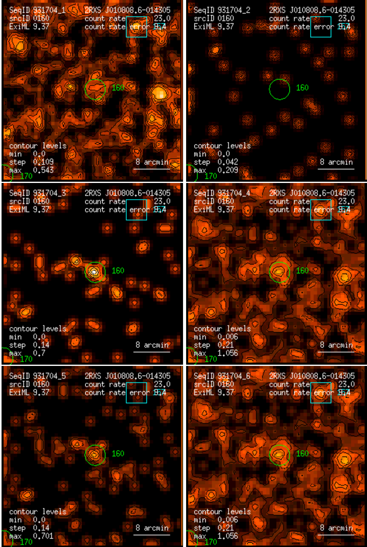
Figure 160: RASS 931704: detection 0160: band rate images, Gaussian filter: (1) PSPC channels 11 – 41, (2) 52 – 90, (3) 91 – 201, (4) 11 – 235, (5) 52 – 201, (6) 11 – 201. Broad band rates in counts/ks. Band rate contour levels in counts/ks/arcmin 2 .
