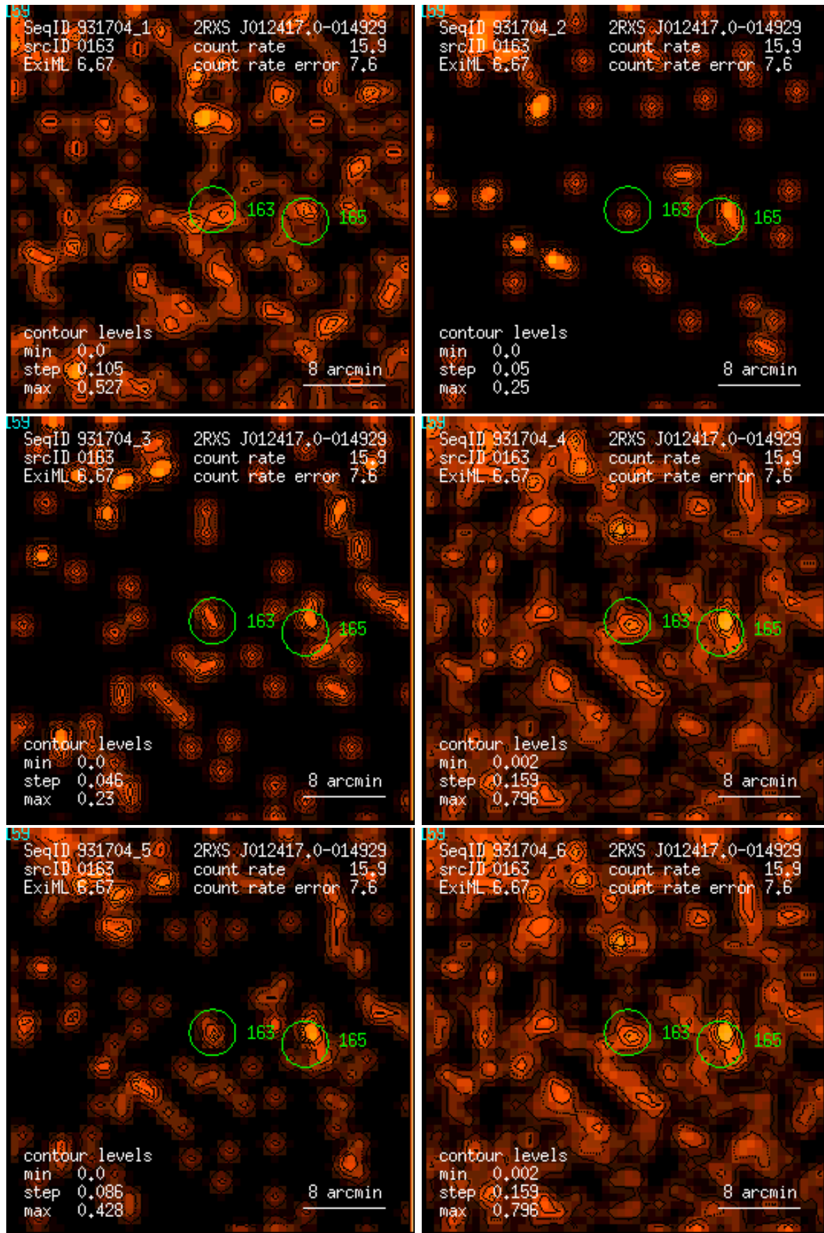
Figure 163: RASS 931704: detection 0163: band rate images, Gaussian filter: (1) PSPC channels 11 – 41, (2) 52 – 90, (3) 91 – 201, (4) 11 – 235, (5) 52 – 201, (6) 11 – 201. Broad band rates in counts/ks. Band rate contour levels in counts/ks/arcmin 2 .
