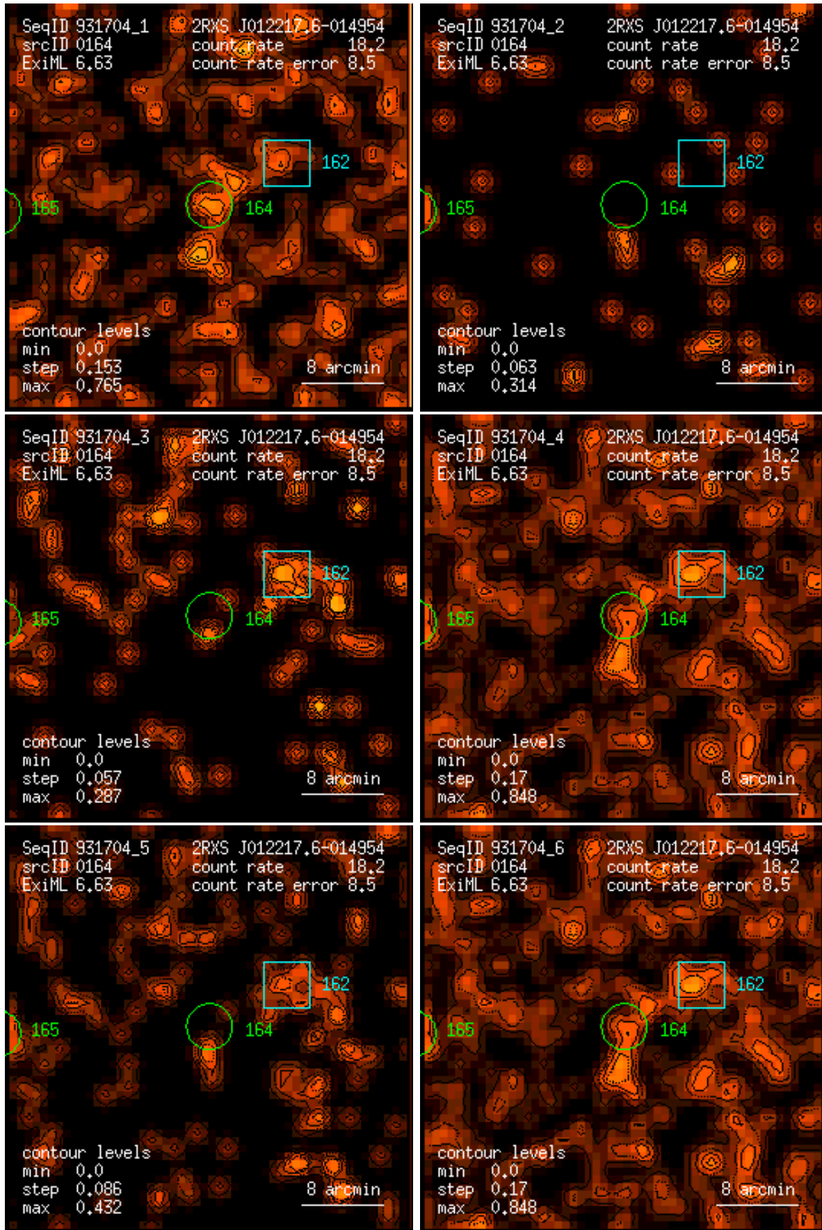
Figure 164: RASS 931704: detection 0164: band rate images, Gaussian filter: (1) PSPC channels 11 – 41, (2) 52 – 90, (3) 91 – 201, (4) 11 – 235, (5) 52 – 201, (6) 11 – 201. Broad band rates in counts/ks. Band rate contour levels in counts/ks/arcmin 2 .
