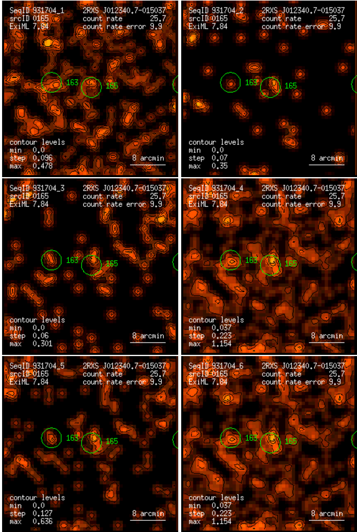
Figure 165: RASS 931704: detection 0165: band rate images, Gaussian filter: (1) PSPC channels 11 – 41, (2) 52 – 90, (3) 91 – 201, (4) 11 – 235, (5) 52 – 201, (6) 11 – 201. Broad band rates in counts/ks. Band rate contour levels in counts/ks/arcmin 2 .
