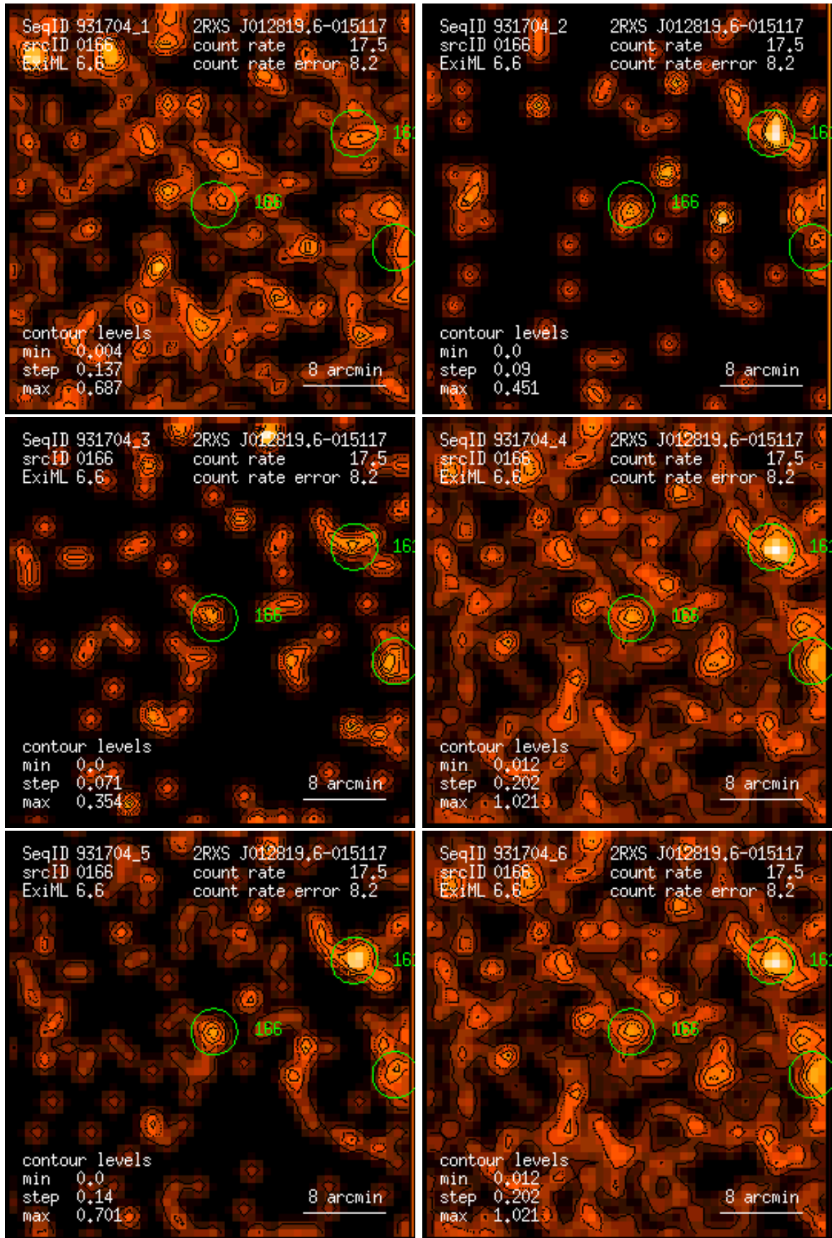
Figure 166: RASS 931704: detection 0166: band rate images, Gaussian filter: (1) PSPC channels 11 – 41, (2) 52 – 90, (3) 91 – 201, (4) 11 – 235, (5) 52 – 201, (6) 11 – 201. Broad band rates in counts/ks. Band rate contour levels in counts/ks/arcmin 2 .
