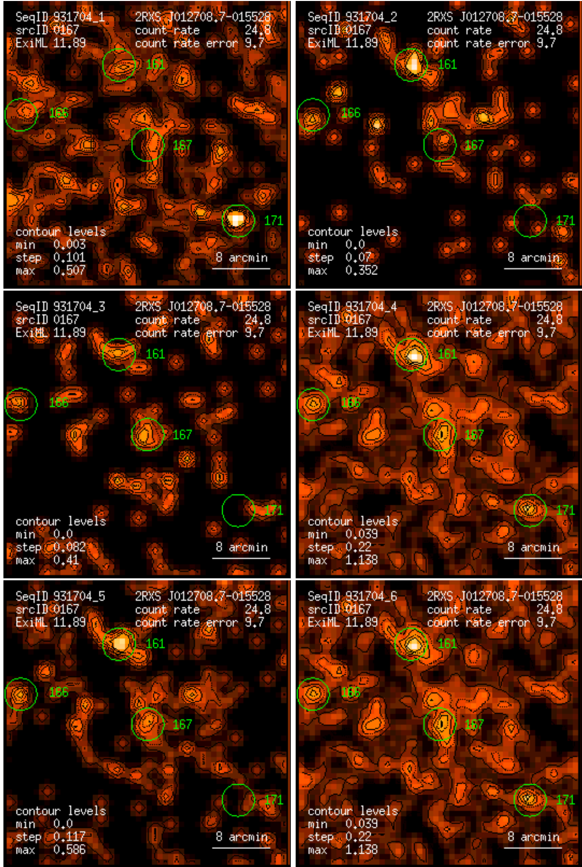
Figure 167: RASS 931704: detection 0167: band rate images, Gaussian filter: (1) PSPC channels 11 – 41, (2) 52 – 90, (3) 91 – 201, (4) 11 – 235, (5) 52 – 201, (6) 11 – 201. Broad band rates in counts/ks. Band rate contour levels in counts/ks/arcmin 2 .
