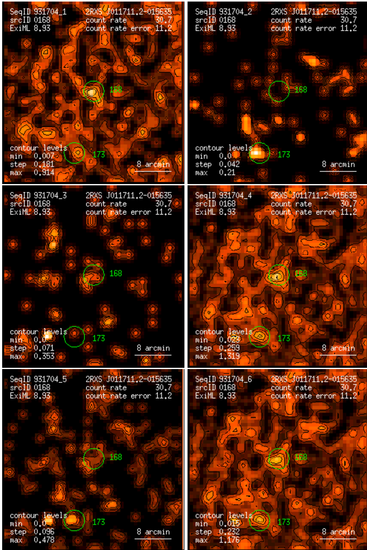
Figure 168: RASS 931704: detection 0168: band rate images, Gaussian filter: (1) PSPC channels 11 – 41, (2) 52 – 90, (3) 91 – 201, (4) 11 – 235, (5) 52 – 201, (6) 11 – 201. Broad band rates in counts/ks. Band rate contour levels in counts/ks/arcmin 2 .
