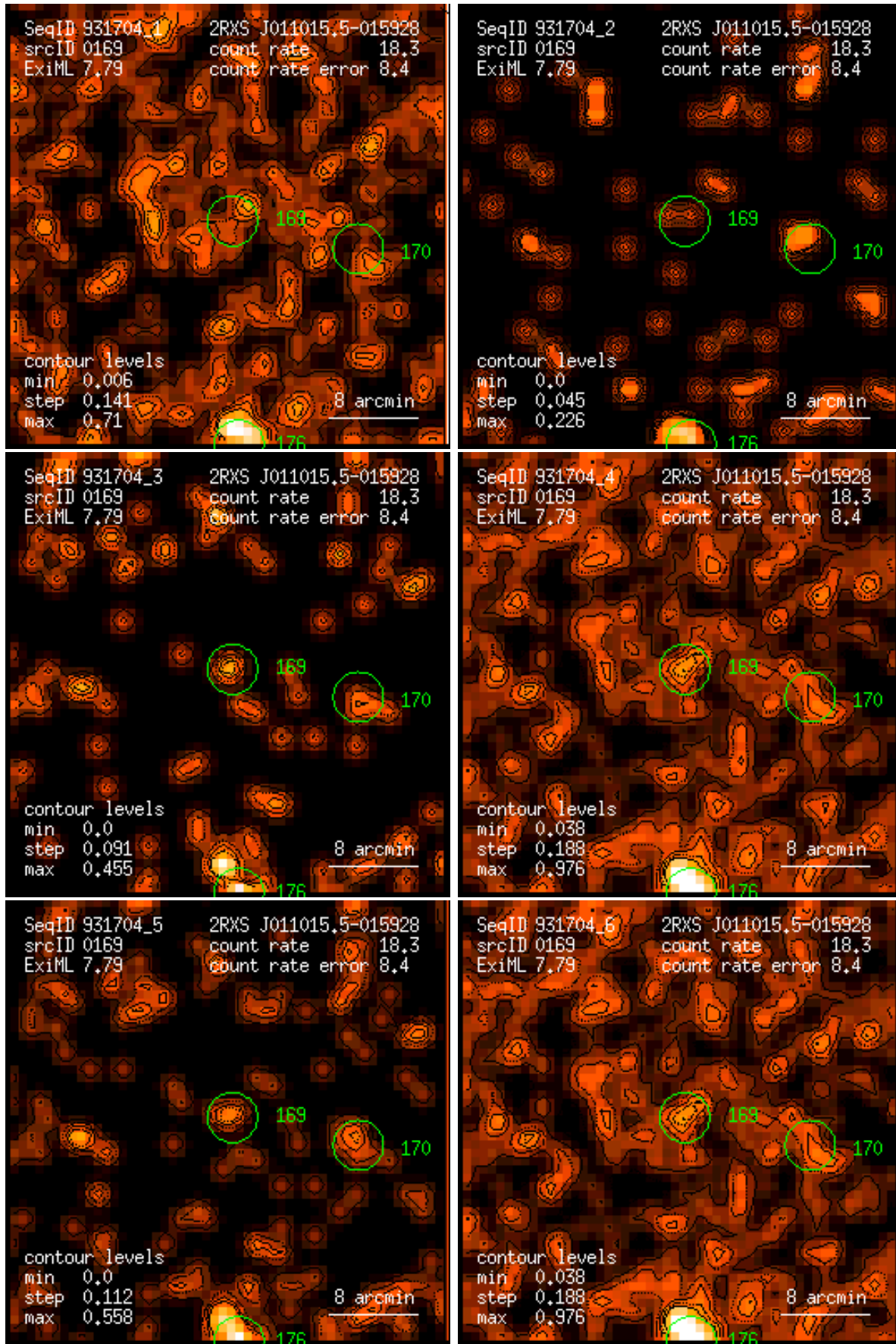
Figure 169: RASS 931704: detection 0169: band rate images, Gaussian filter: (1) PSPC channels 11 – 41, (2) 52 – 90, (3) 91 – 201, (4) 11 – 235, (5) 52 – 201, (6) 11 – 201. Broad band rates in counts/ks. Band rate contour levels in counts/ks/arcmin 2 .
