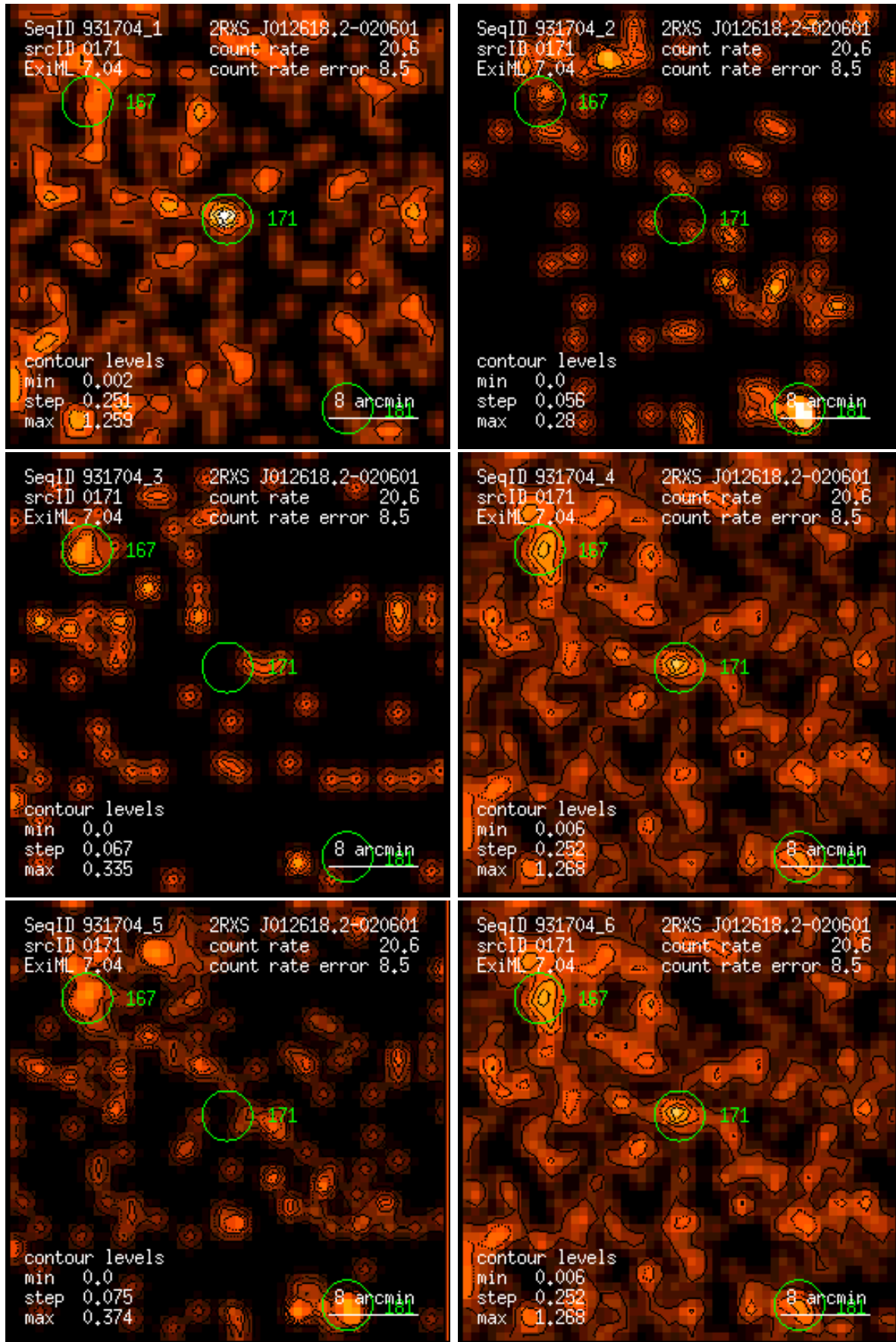
Figure 171: RASS 931704: detection 0171: band rate images, Gaussian filter: (1) PSPC channels 11 – 41, (2) 52 – 90, (3) 91 – 201, (4) 11 – 235, (5) 52 – 201, (6) 11 – 201. Broad band rates in counts/ks. Band rate contour levels in counts/ks/arcmin 2 .
