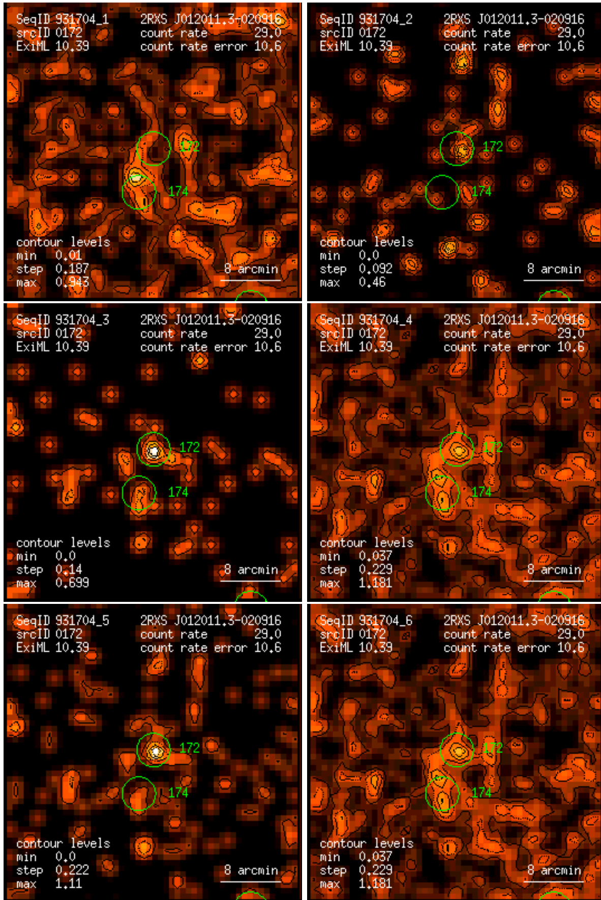
Figure 172: RASS 931704: detection 0172: band rate images, Gaussian filter: (1) PSPC channels 11 – 41, (2) 52 – 90, (3) 91 – 201, (4) 11 – 235, (5) 52 – 201, (6) 11 – 201. Broad band rates in counts/ks. Band rate contour levels in counts/ks/arcmin 2 .
