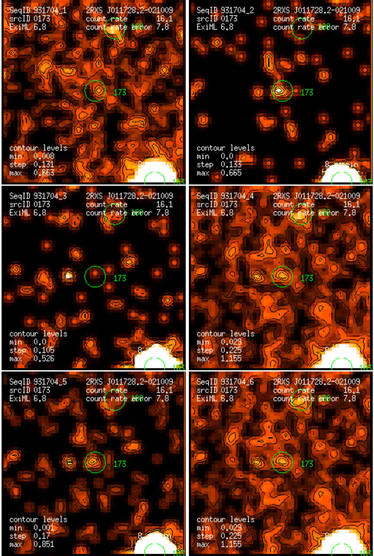
Figure 173: RASS 931704: detection 0173: band rate images, Gaussian filter: (1) PSPC channels 11 – 41, (2) 52 – 90, (3) 91 – 201, (4) 11 – 235, (5) 52 – 201, (6) 11 – 201. Broad band rates in counts/ks. Band rate contour levels in counts/ks/arcmin 2 .
