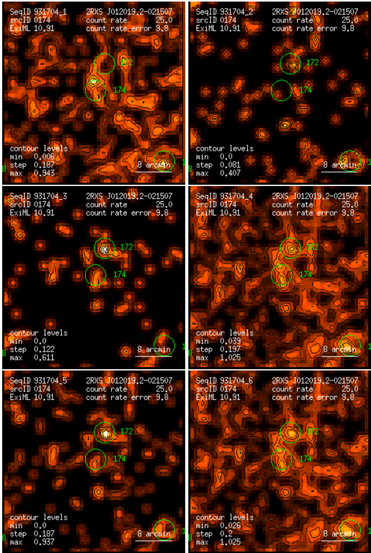
Figure 174: RASS 931704: detection 0174: band rate images, Gaussian filter: (1) PSPC channels 11 – 41, (2) 52 – 90, (3) 91 – 201, (4) 11 – 235, (5) 52 – 201, (6) 11 – 201. Broad band rates in counts/ks. Band rate contour levels in counts/ks/arcmin 2 .
