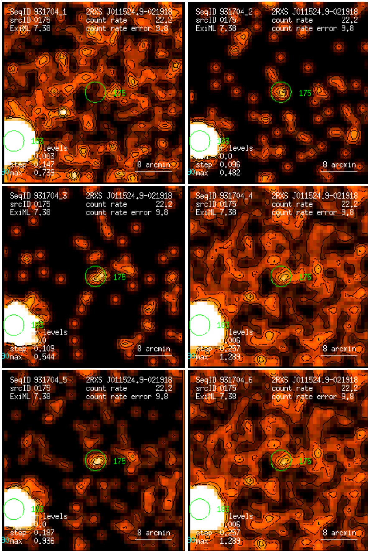
Figure 175: RASS 931704: detection 0175: band rate images, Gaussian filter: (1) PSPC channels 11 – 41, (2) 52 – 90, (3) 91 – 201, (4) 11 – 235, (5) 52 – 201, (6) 11 – 201. Broad band rates in counts/ks. Band rate contour levels in counts/ks/arcmin 2 .
