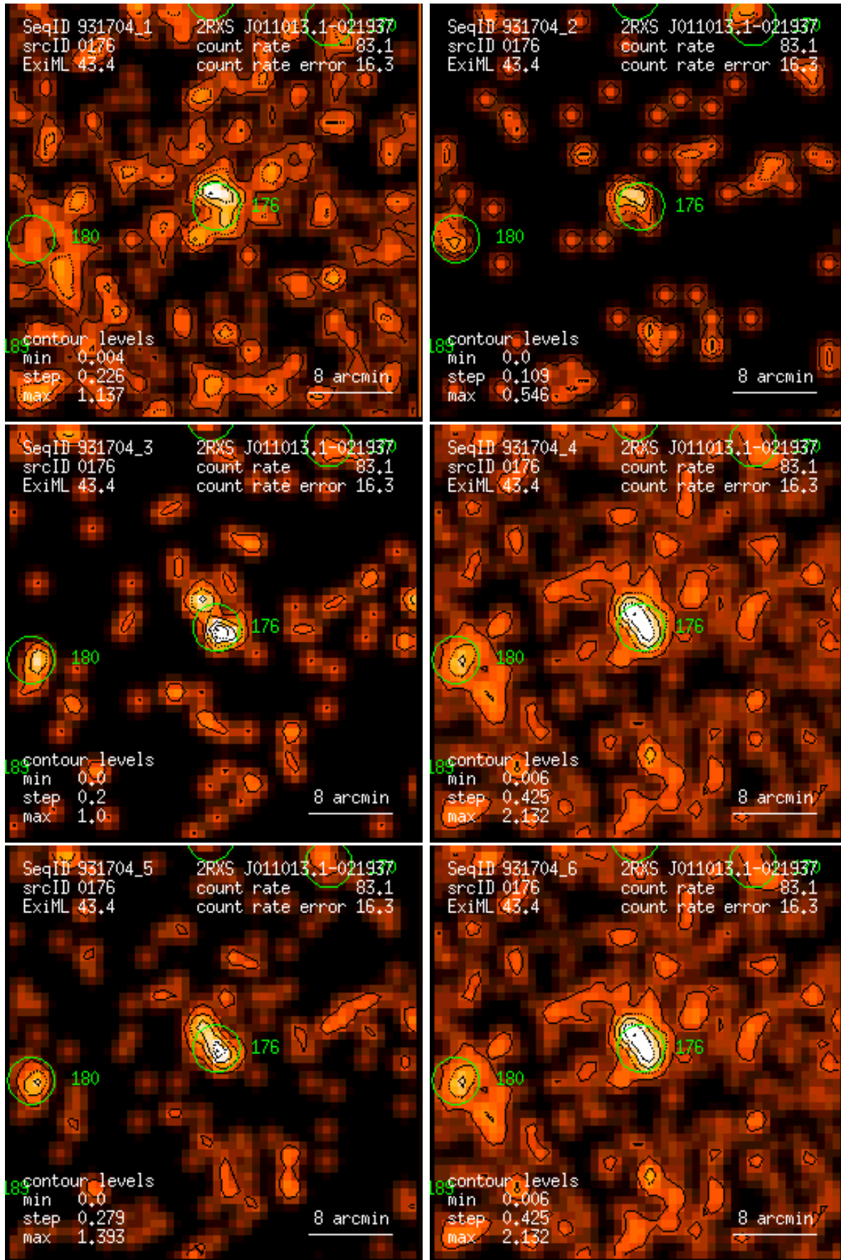
Figure 176: RASS 931704: detection 0176: band rate images, Gaussian filter: (1) PSPC channels 11 – 41, (2) 52 – 90, (3) 91 – 201, (4) 11 – 235, (5) 52 – 201, (6) 11 – 201. Broad band rates in counts/ks. Band rate contour levels in counts/ks/arcmin 2 .
