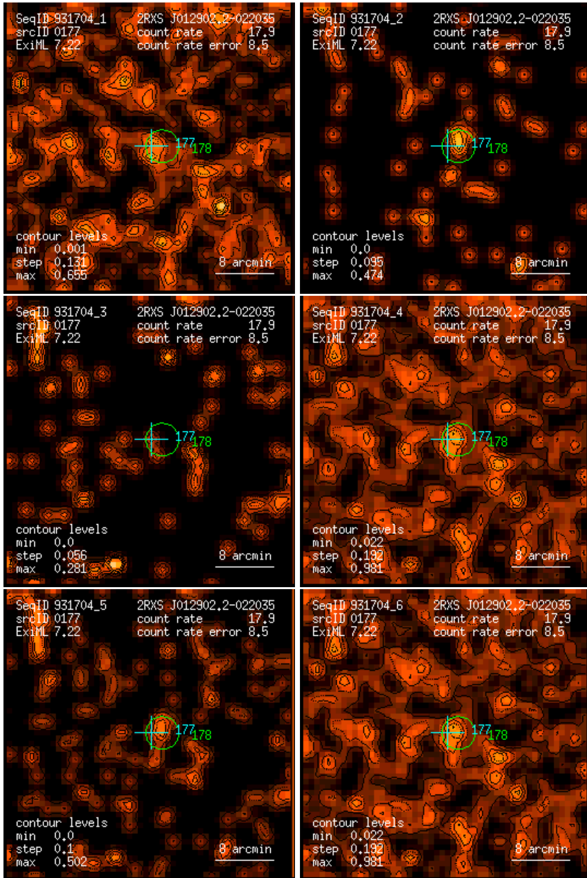
Figure 177: RASS 931704: detection 0177: band rate images, Gaussian filter: (1) PSPC channels 11 – 41, (2) 52 – 90, (3) 91 – 201, (4) 11 – 235, (5) 52 – 201, (6) 11 – 201. Broad band rates in counts/ks. Band rate contour levels in counts/ks/arcmin 2 .
