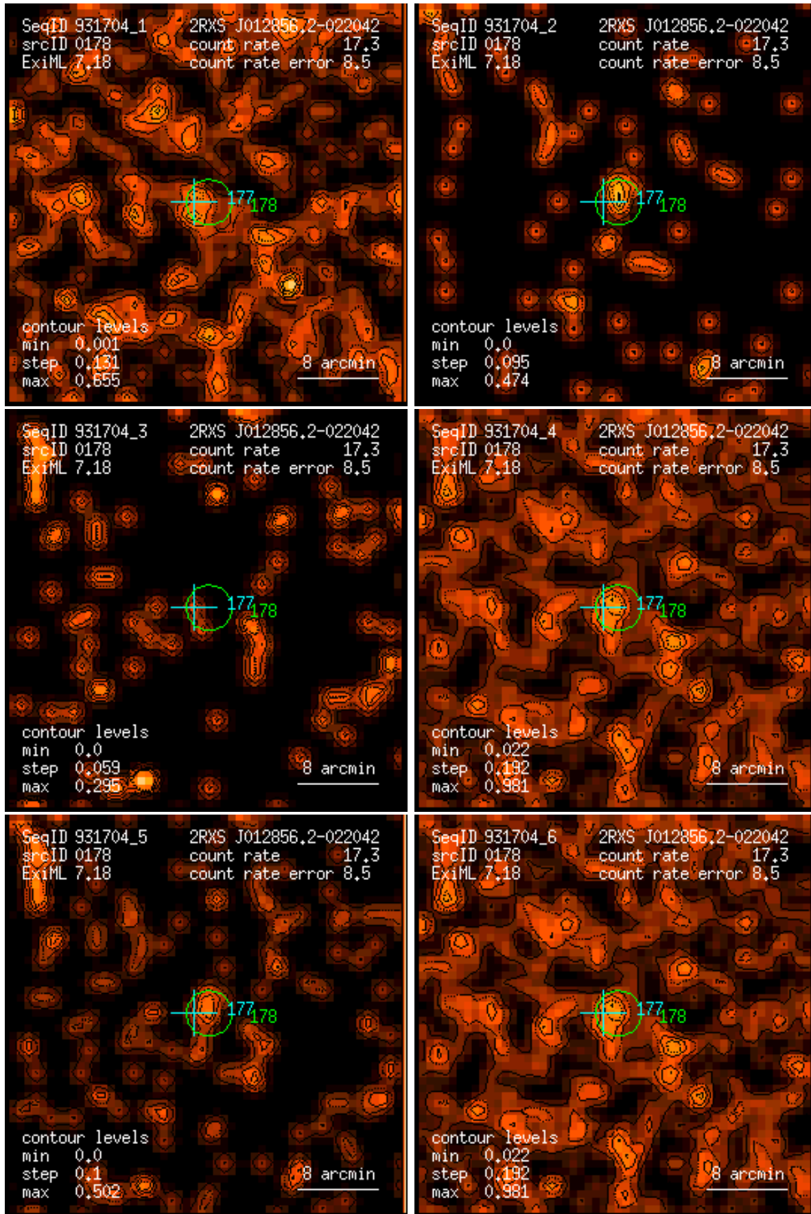
Figure 178: RASS 931704: detection 0178: band rate images, Gaussian filter: (1) PSPC channels 11 – 41, (2) 52 – 90, (3) 91 – 201, (4) 11 – 235, (5) 52 – 201, (6) 11 – 201. Broad band rates in counts/ks. Band rate contour levels in counts/ks/arcmin 2 .
