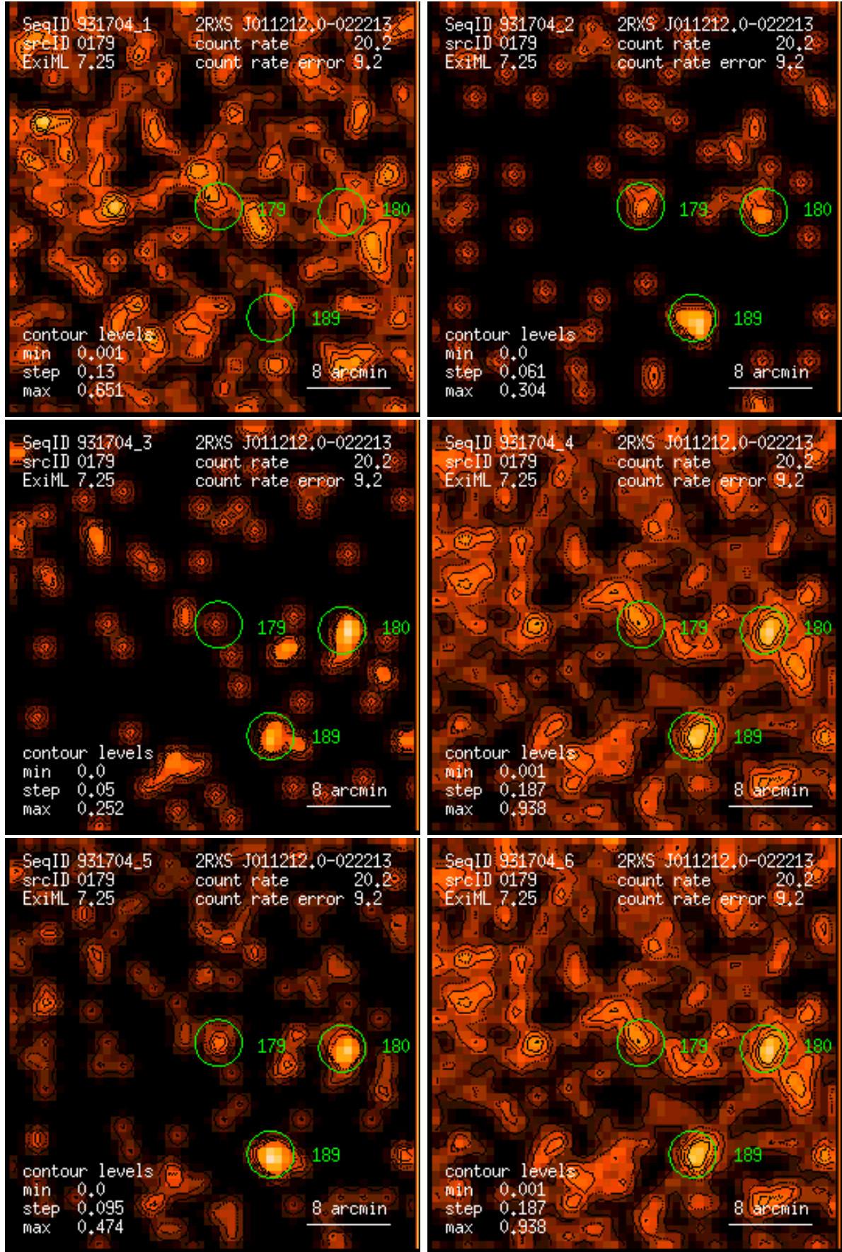
Figure 179: RASS 931704: detection 0179: band rate images, Gaussian filter: (1) PSPC channels 11 – 41, (2) 52 – 90, (3) 91 – 201, (4) 11 – 235, (5) 52 – 201, (6) 11 – 201. Broad band rates in counts/ks. Band rate contour levels in counts/ks/arcmin 2 .
