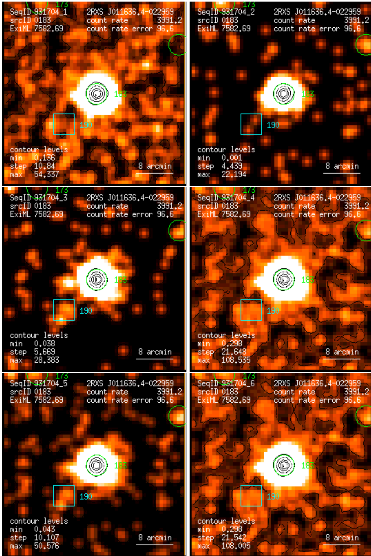
Figure 183: RASS 931704: detection 0183: band rate images, Gaussian filter: (1) PSPC channels 11 – 41, (2) 52 – 90, (3) 91 – 201, (4) 11 – 235, (5) 52 – 201, (6) 11 – 201. Broad band rates in counts/ks. Band rate contour levels in counts/ks/arcmin 2 .
