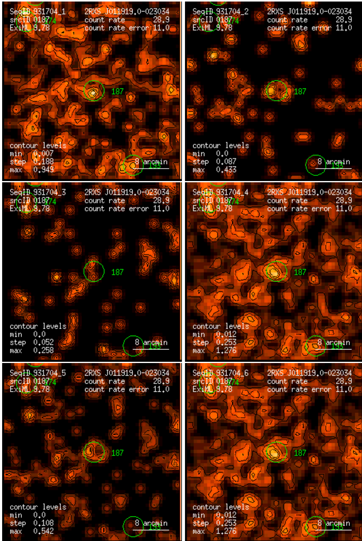
Figure 187: RASS 931704: detection 0187: band rate images, Gaussian filter: (1) PSPC channels 11 – 41, (2) 52 – 90, (3) 91 – 201, (4) 11 – 235, (5) 52 – 201, (6) 11 – 201. Broad band rates in counts/ks. Band rate contour levels in counts/ks/arcmin 2 .
