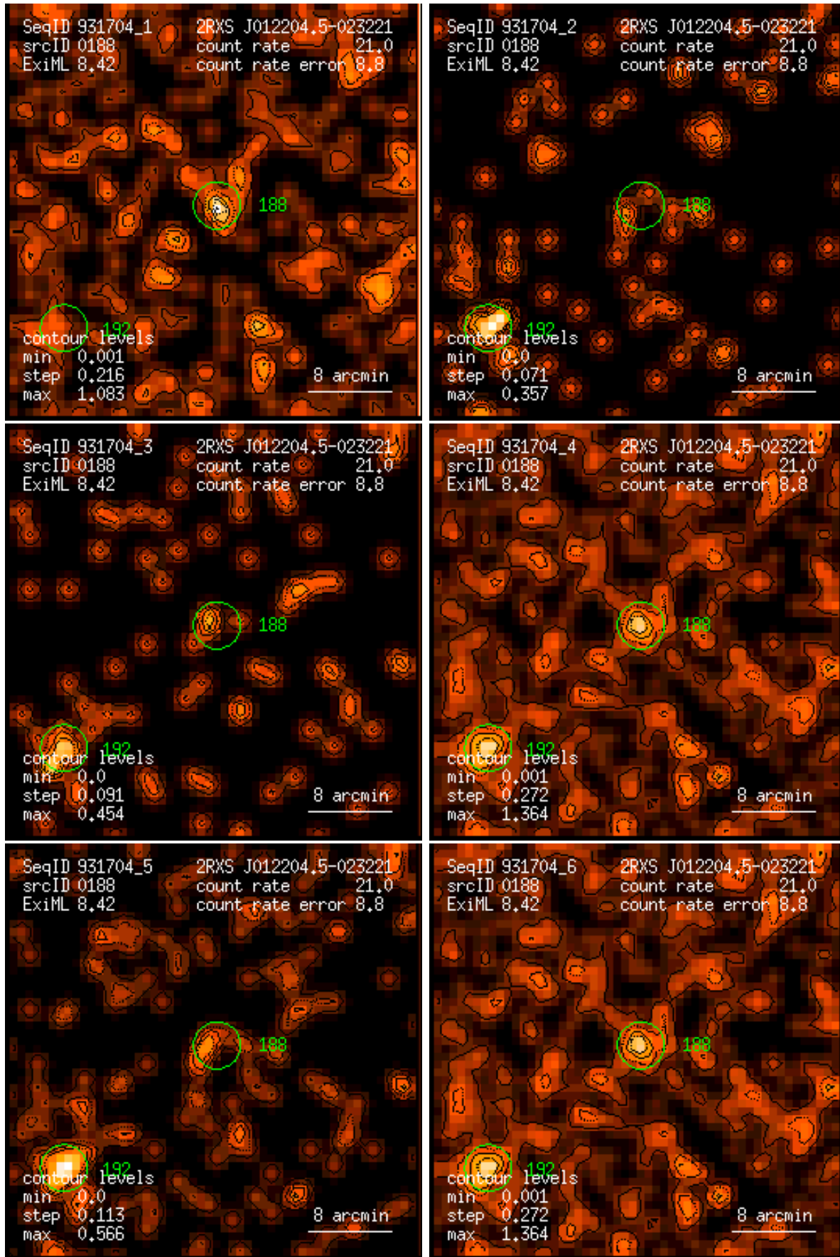
Figure 188: RASS 931704: detection 0188: band rate images, Gaussian filter: (1) PSPC channels 11 – 41, (2) 52 – 90, (3) 91 – 201, (4) 11 – 235, (5) 52 – 201, (6) 11 – 201. Broad band rates in counts/ks. Band rate contour levels in counts/ks/arcmin 2 .
